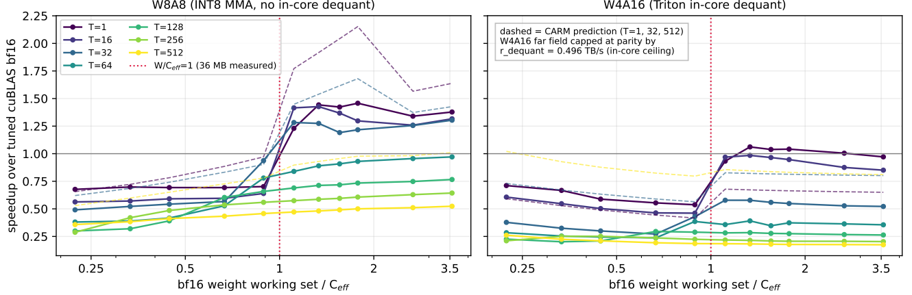
Figure 1: The capacity gate. Speedup over tuned cuBLAS bf16 vs. normalized weight working set W/C_{\text{eff}} , one line per token count T ; 77 cells, clock-locked, CUDA-graph timed (10 launches/graph, median of 30 replays), per-cell mini-autotuned. At decode-scale T \leq 32 the sign flips between W=32 and 40 MB — bracketing the measured C_{\text{eff}}=36 MB. W8A8 (left; INT8 MMA, dynamic act-quant inside the timed region, no in-core dequant) reaches 1.2–1.46 \times in the far field; W4A16 (right) flips at the same boundary but caps at parity, bound by its in-core dequant ceiling. At T \geq 64 both lose everywhere: the compute-bound regime that produces MARLIN’s reported batch-64 collapse. Data: profiling/gate/results-capacity-gate.json.
