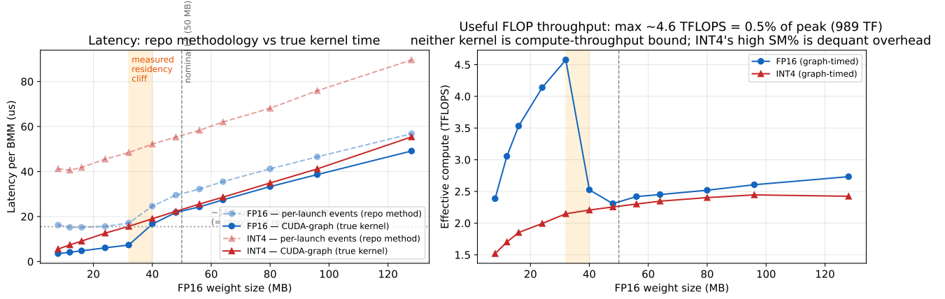
Figure 5: Methodology validation (H100, bs=1, audit stack: torch 2.7/triton 3.3). Left: per-launch event timing (repo method, dashed) vs. CUDA-graph timing (true kernel, solid). The \sim 15.5 \mu s launch/eventing floor — not L2 serving — produces the apparent flat region below 32 MB; true kernel latency scales with weight size. Right: effective compute throughput peaks at \sim 4.6 TFLOPS, 0.5% of the 989 TF peak, so neither kernel is compute-throughput-bound and INT4's high SM utilization is dequantization overhead, not useful FLOPs. Orange band: measured 32–40 MB residency cliff; dashed line: nominal 50 MB L2.
