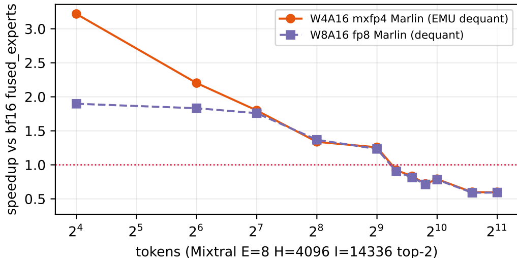
H100 — every FP4 path must dequantize (no FP4 tensor cores)
