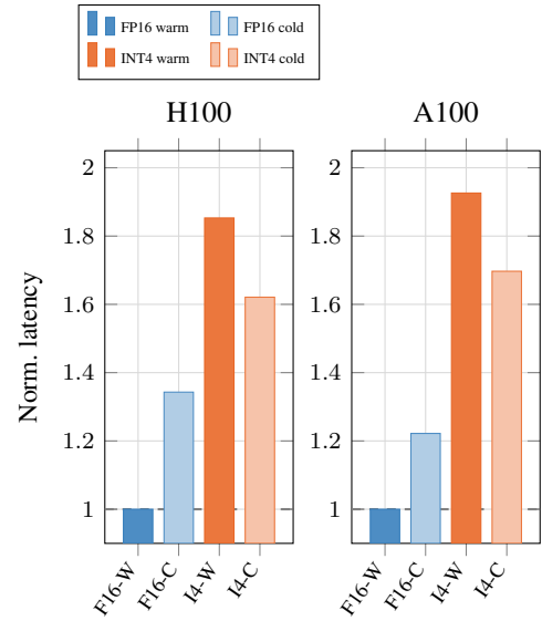
Figure 4: Cache-residency intervention at fixed MLA reconstruction shape (BS=1, normalized to FP16-warm). H100: eviction adds +4.8\ \mu\text{s} to FP16 (= full 16 MB weight reload at HBM rate) and +3.9\ \mu\text{s} to INT4, of which \sim 2.6\ \mu\text{s} is common-mode eviction overhead (expected INT4 reload: 1.3\ \mu\text{s} ). The FP16 delta supports L2-residency dependence of the FP16 path; note that absolute deltas, not relative percentages, are the comparable quantity here since the two baselines differ \sim 2.6\times .
