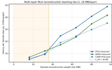
Figure 11: Multi-layer MLA reconstruction stacking (bs=1, 16 MB/layer, graph-timed). Stacking 1–6 layers sweeps the per-step working set from 16 to 96 MB; the FP16→W8A8 crossover occurs between two and three layers (32→48 MB), bracketing the measured C_{\text{eff}} \approx 36 MB. Dashed: CARM FP16 prediction.
