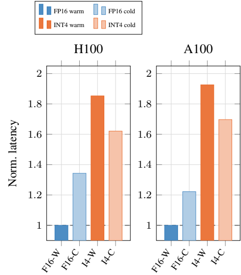
Figure 5: Cache-residency intervention at fixed MLA reconstruction shape (BS=1, normalized to FP16-warm). H100: eviction adds +4.8 \mu\text{s} to FP16 (= full 16 MB weight reload at HBM rate) and +3.9 \mu\text{s} to INT4, of which \sim 2.6 \mu\text{s} is common-mode eviction overhead (expected INT4 reload: 1.3 \mu\text{s} ). The FP16 delta supports L2-residency dependence of the FP16 path; note that absolute deltas, not relative percentages, are the comparable quantity here since the two baselines differ \sim 2.6\times .
