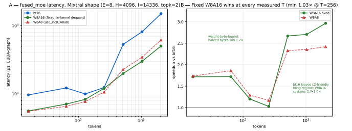
Figure 12: FlagGems fused_moe, Mixtral shape, graph-timed (T=16–2048). A : latency for bf16, fixed W8A16 (in-kernel dequant), and W8A8. B : speedup over bf16 — the fixed W8A16 kernel wins at every measured token count, 2.7–3.0 \times at T \geq 512 .
