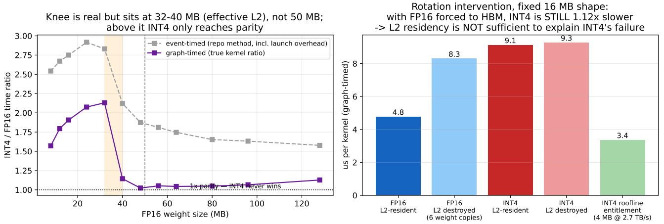
Figure 8: INT4/FP16 ratio and causal decomposition (H100, bs=1, audit stack). Left: INT4/FP16 time ratio vs. weight size, event-timed (grey, launch-overhead-inflated) and graph-timed (purple, true kernel). The knee sits at the measured 32–40 MB effective capacity, not the nominal 50 MB; the graph-timed kernel ratio ( 1.9\times near the cliff \rightarrow 1.0\text{--}1.1\times at 128 MB) matches the main-stack result, while event-timed magnitudes are stack-dependent (a robustness caveat we flag in the Limitations). Right: weight-rotation intervention at fixed 16 MB shape. Forcing FP16 out of L2 (6 weight copies) raises FP16 from 4.8 to 8.3 \mu\text{s} , but INT4 (9.1–9.3 \mu\text{s} , cache-insensitive) is still 1.12\times slower than evicted FP16 and runs 2.7\times above its \sim 3.4\ \mu\text{s} memory entitlement: L2 residency is necessary but not sufficient to explain INT4’s failure; dequantization compute accounts for the rest.
