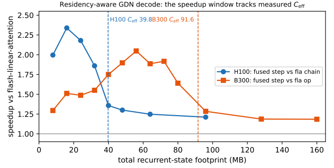
Figure 4: The residency-aware GDN decode kernel’s speedup window tracks measured C_{\text{eff}} across architectures. Speedup over flash-linear-attention vs. total recurrent-state footprint (H100: vs. the practical 3-kernel decode chain; B300: vs. the fused-recurrent op). Each curve collapses at its own card’s independently measured effective capacity (dashed) — 39.8 MB on H100, 91.6 MB on B300 — locations predicted before the kernel ran on either card. The \geq 1.2\times far-field floor is the kernel-fusion dividend. Data: explorations/state_residency/ .
