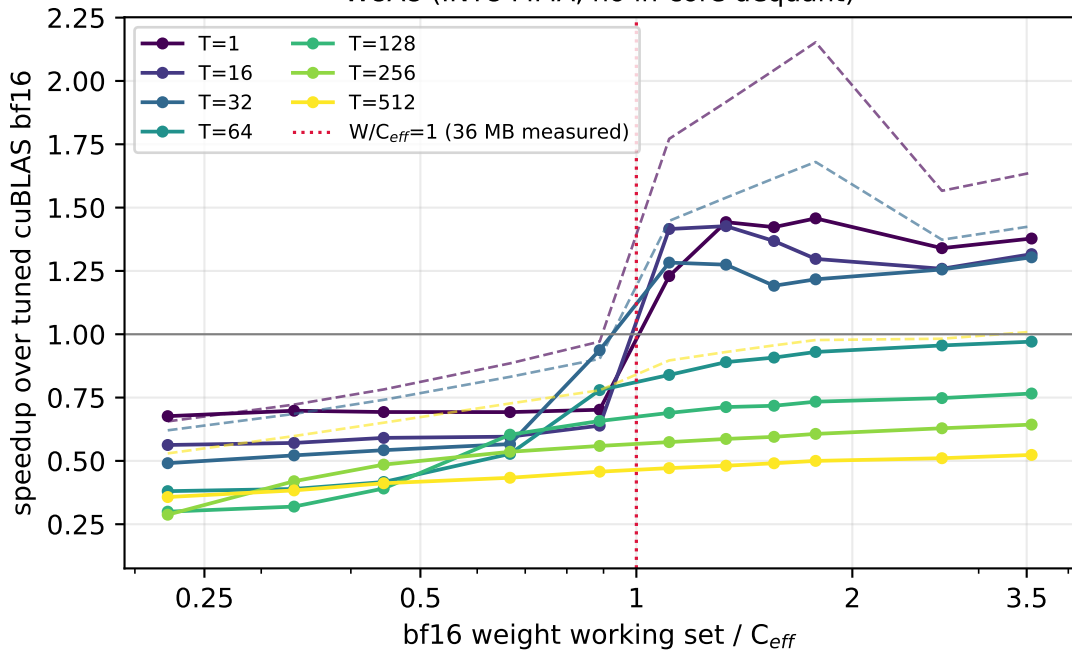
W8A8 (INT8 MMA, no in-core dequant)
