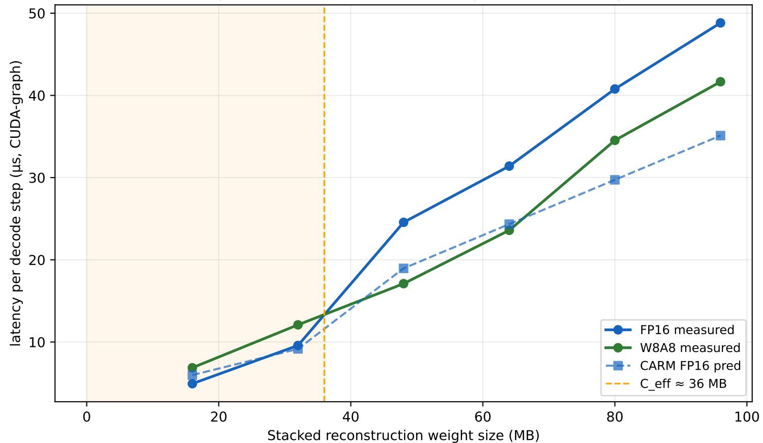
Multi-layer MLA reconstruction stacking (bs=1, 16 MB/layer)
