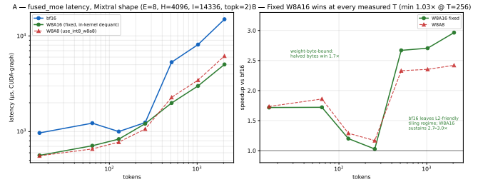
Figure 11: FlagGems fused_moe, Mixtral shape, graph-timed (T=16–2048). A : latency for bf16, fixed W8A16 (in-kernel dequant), and W8A8. B : speedup over bf16 — the fixed W8A16 kernel wins at every measured token count, 2.7–3.0× at T≥512.
