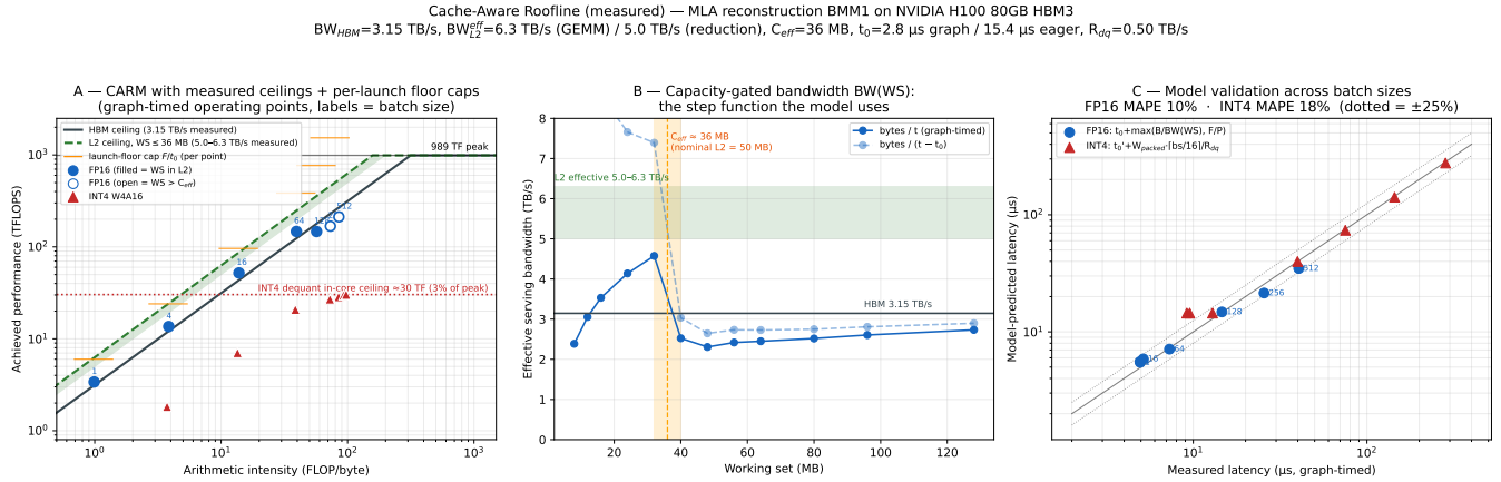
Figure 8: Measured cache-aware roofline for MLA reconstruction (H100, graph-timed). A: CARM with measured HBM and L2 ceilings, per-point launch-floor caps, and the fitted INT4 dequant in-core ceiling ( \sim 30 TF); FP16 points (labeled by batch size) are filled when the working set fits C_{eff} . B: the capacity-gated bandwidth function BW(WS) — effective serving bandwidth vs. working set, with the measured residency cliff at 32–40 MB. C: model validation, predicted vs. measured latency (dotted = \pm 25\% ).
