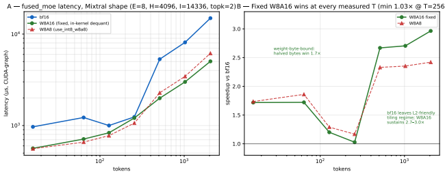
Figure 11: FlagGems fused_moe, Mixtral shape, graph-timed ( T=16 –2048). A : latency for bf16, fixed W8A16 (in-kernel dequant), and W8A8. B : speedup over bf16 — the fixed W8A16 kernel wins at every measured token count, 2.7 – 3.0\times at T\geq 512 .
