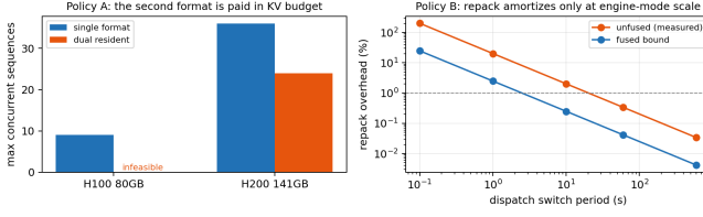
Figure 3: Storage policies for runtime precision dispatch (27B dense model, p32768d1024). Left: holding a second weight format is paid out of the KV budget — infeasible on 80 GB, \sim 33\% concurrency on H200 141 GB. Right: repacking on a dispatch switch amortizes below 1% overhead only at \geq 20 s (measured unfused) / \geq 2.5 s (fused bound) switch periods. Data: profiling/dispatch/results_cost_model.json .
