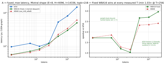
Figure 11: FlagGems fused_moe , Mixtral shape, graph-timed (T=16–2048). A : latency for bf16, fixed W8A16 (in-kernel dequant), and W8A8. B : speedup over bf16 — the fixed W8A16 kernel wins at every measured token count, 2.7–3.0 \times at T \geq 512.
