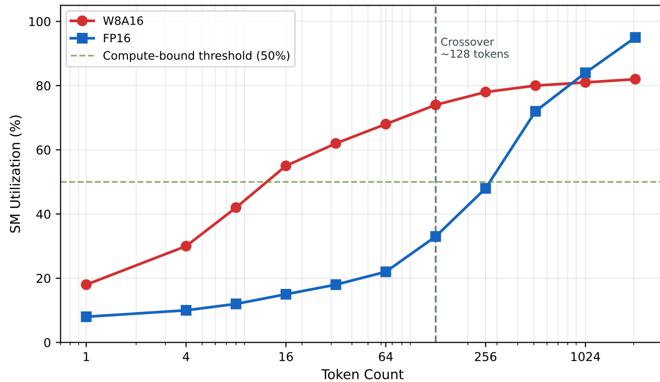
(C) SM Compute Utilization (kernel-compass)
