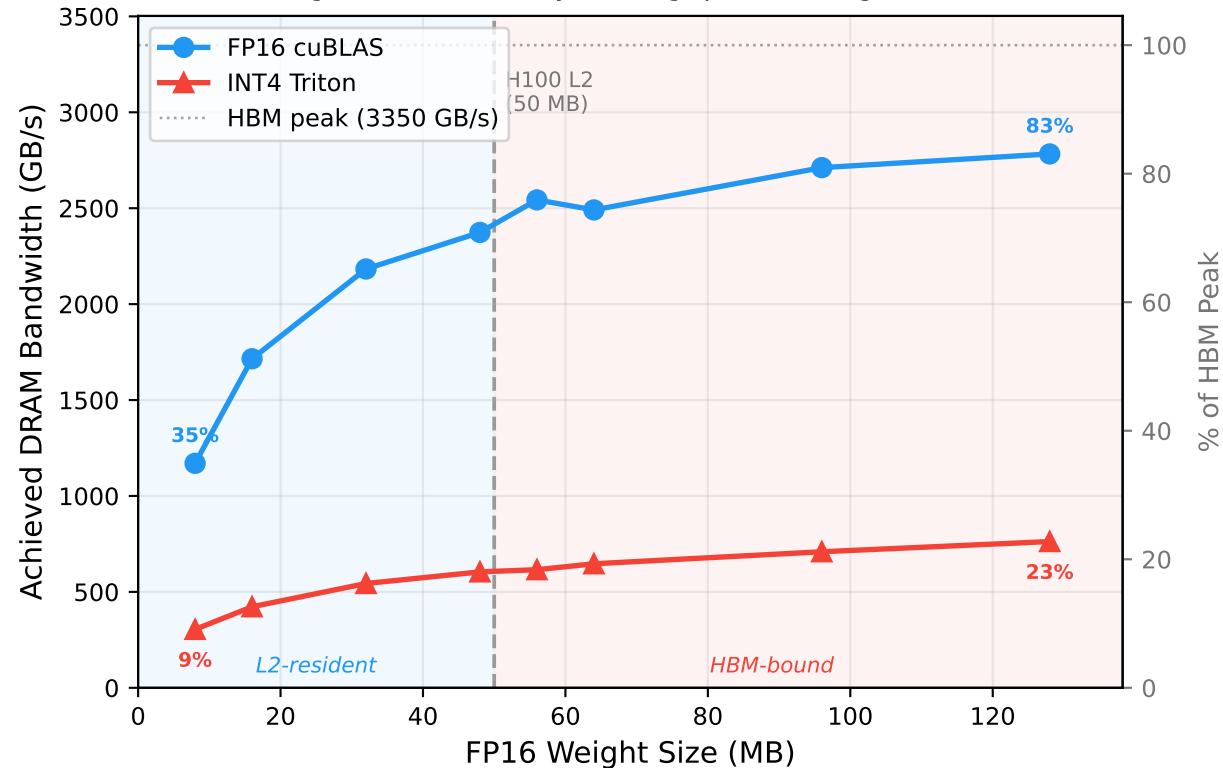
Figure A — Memory Throughput vs Weight Size
