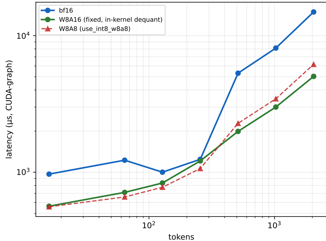
A — fused_moe latency, Mixtral shape (E=8, H=4096, l=14336, topk=2) B — Fixed W8A16 wins at every measured T (min 1.03x @ T=256)
