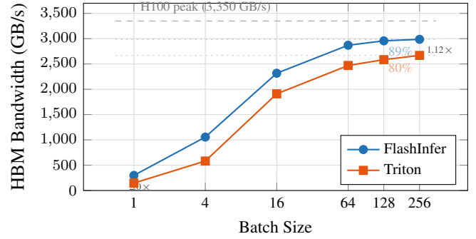
Figure 1: Decode bandwidth vs. batch size (Llama-3-8B, L_{kv}=2048 ). Both backends approach HBM saturation; FlashInfer peaks at 89% of H100 peak. The gap narrows from 2 \times at bs=1 to 1.12 \times at bs=256 as launch overhead becomes negligible relative to streaming KV reads.
