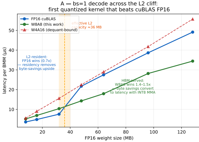
Figure 10: W8A8 INT8-MMA vs. cuBLAS FP16 vs. Triton W4A16 for MLA reconstruction (graph-timed, H100). Left: weight-size sweep at bs=1 ; right: batch-size sweep at 128 MB. Orange band: measured effective L2 capacity ( \sim 36 \text{ MB} ).
