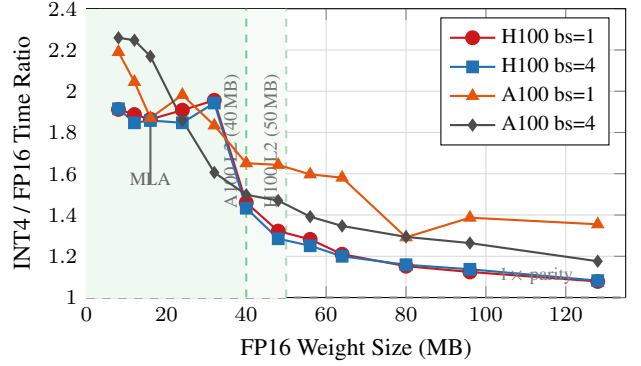
Figure 8: Weight-size scaling on H100 and A100: event-timed INT4/FP16 ratio vs. FP16 weight size. Below the knee INT4 is much slower; above it the ratio moves toward (but never below) parity as FP16 falls back to HBM. Two caveats apply: (i) the H100 knee sits at 32–40 MB, the effective residency capacity measured by warm-state DRAM-read counters, not at the nominal 50 MB; (ii) these event-timed curves embed a \sim 15.5 \mu s per-launch floor that flattens the small-size region — CUDA-graph timing shows the same knee with kernel-level ratios of 1.9\times \rightarrow 1.0\text{--}1.1\times . At MLA’s 16 MB operating point (arrow), both platforms are in the (partially) L2-resident regime.
