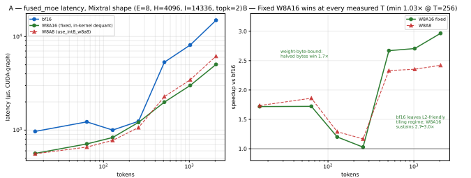
Figure 12: FlagGems fused_moe , Mixtral shape, graph-timed ( T=16\text{--}2048 ). A : latency for bf16, fixed W8A16 (in-kernel dequant), and W8A8. B : speedup over bf16 — the fixed W8A16 kernel wins at every measured token count, 2.7\text{--}3.0\times at T \geq 512 .
