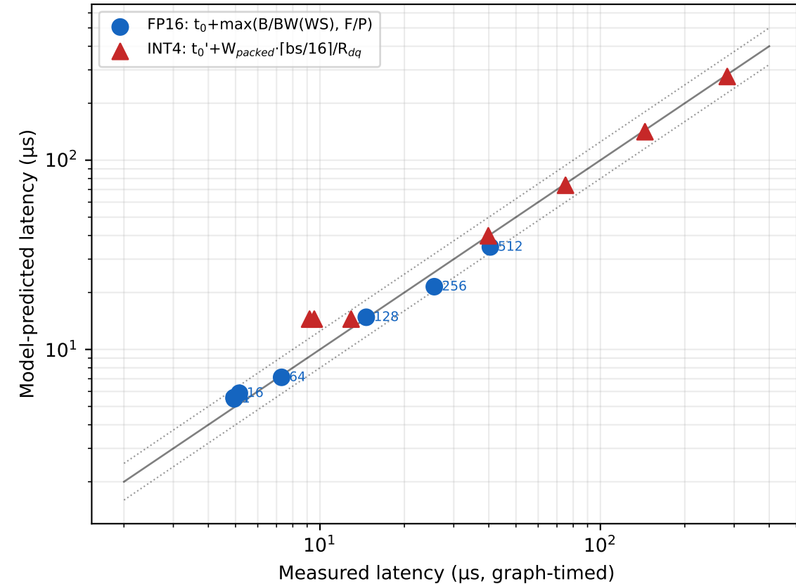
C — Model validation across batch sizes FP16 MAPE 10% · INT4 MAPE 18% (dotted = \pm 25\% )
