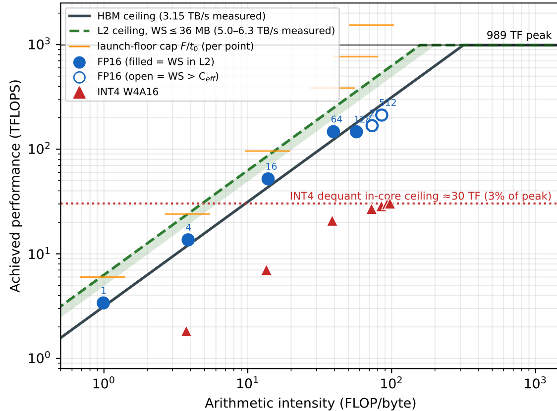
A — CARM with measured ceilings + per-launch floor caps (graph-timed operating points, labels = batch size)
