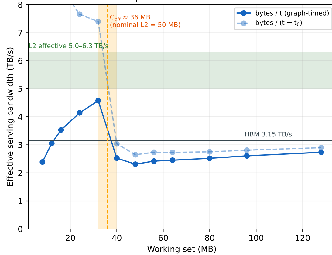
B — Capacity-gated bandwidth BW(WS) : the step function the model uses
