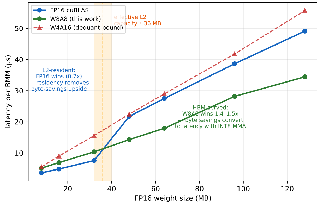
A — bs=1 decode across the L2 cliff: first quantized kernel that beats cuBLAS FP16
