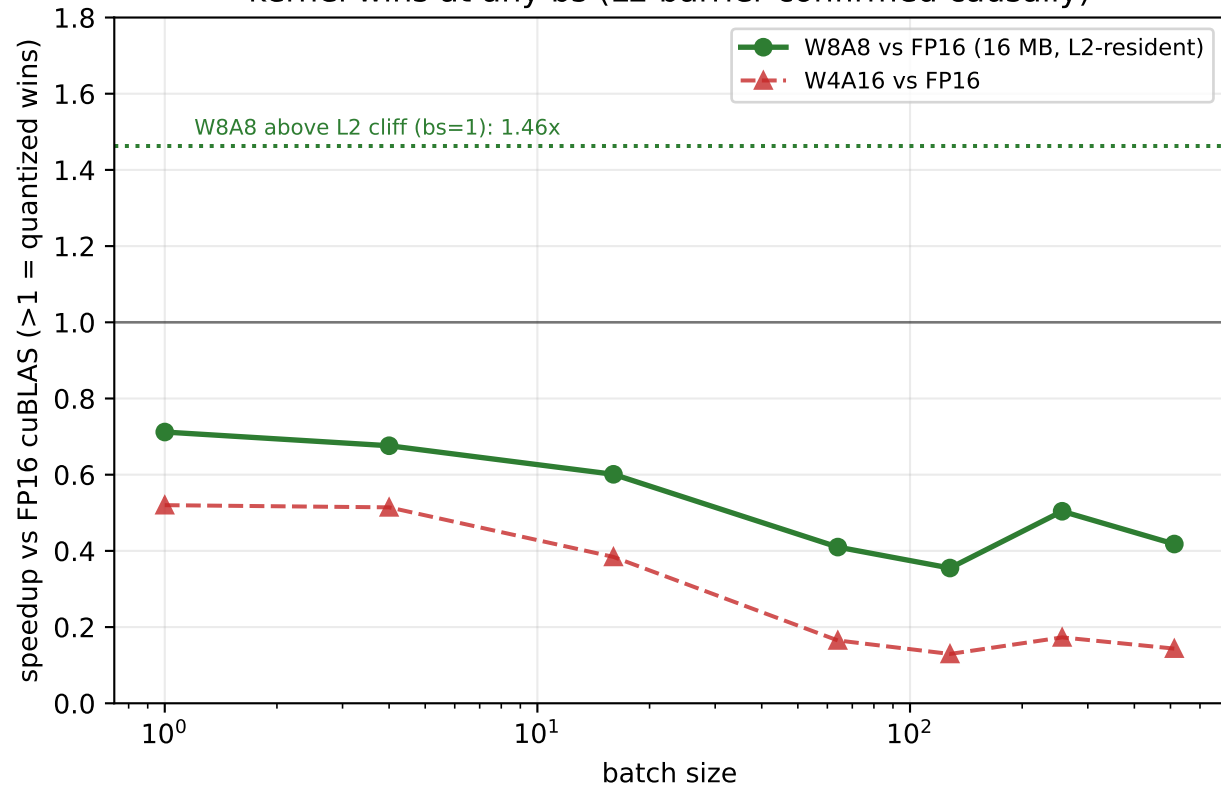
B — at the 16 MB L2-resident MLA shape no quantized kernel wins at any bs (L2 barrier confirmed causally)
