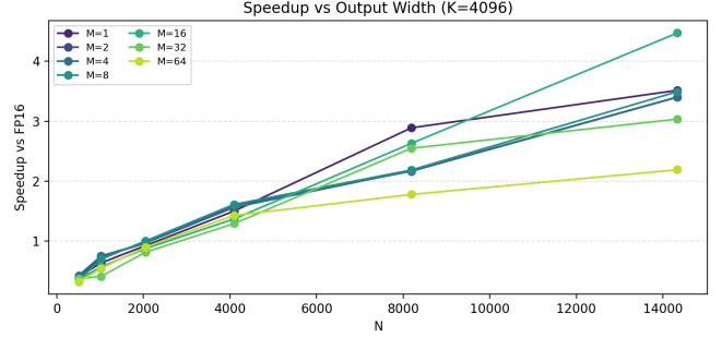
Figure 3: Speedup vs output width N (decode shapes, K = 4096 ).
