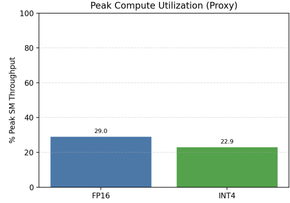
Figure 6: Peak compute utilization proxy (SM throughput) for FP16 vs INT4.
