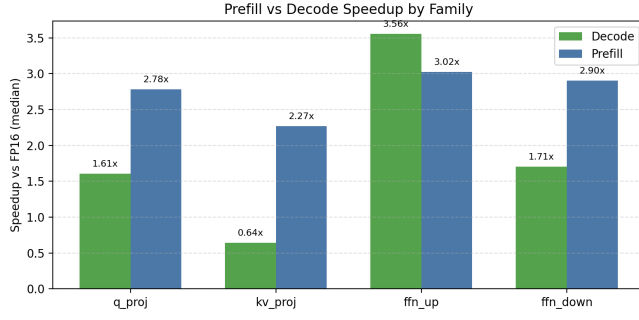
Figure 5: Prefill vs decode speedup by family.
