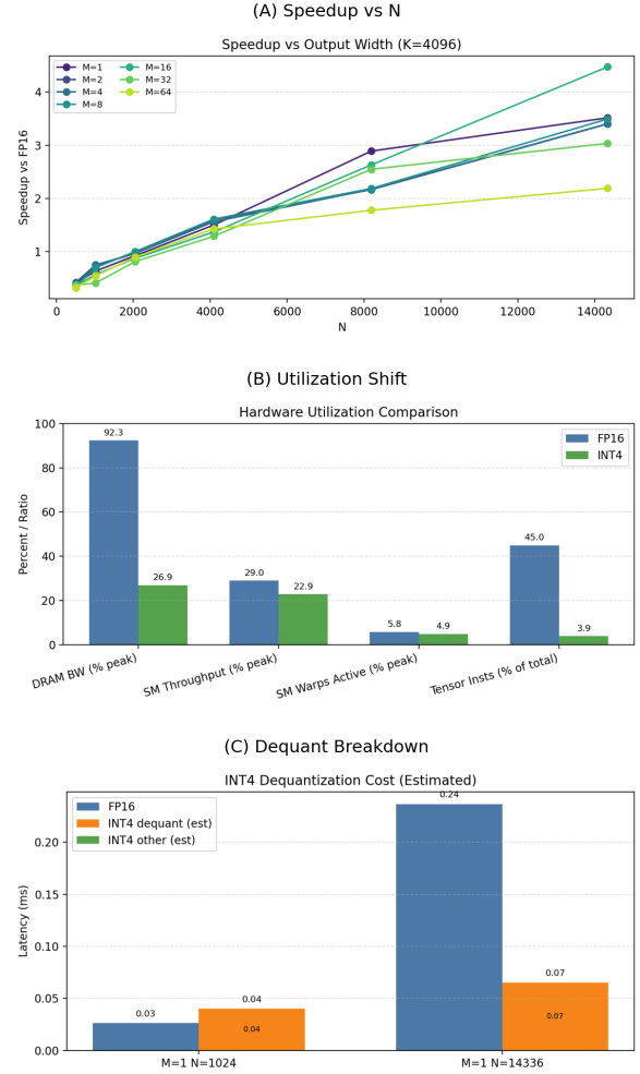
Figure 2: INT4 helps when bandwidth dominates and dequant is amortized.
