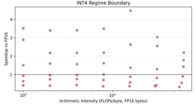
Figure 10: Regime boundary: speedup vs arithmetic intensity.
