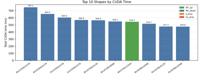
Figure 9: Top shapes by CUDA time (Nsight Systems).
