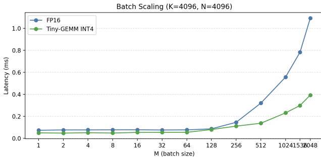
(a) Latency vs batch ( K = N = 4096 ).
