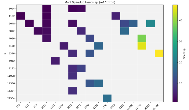
Figure 10: Decode regime map ( M=1 ) across K and N .
