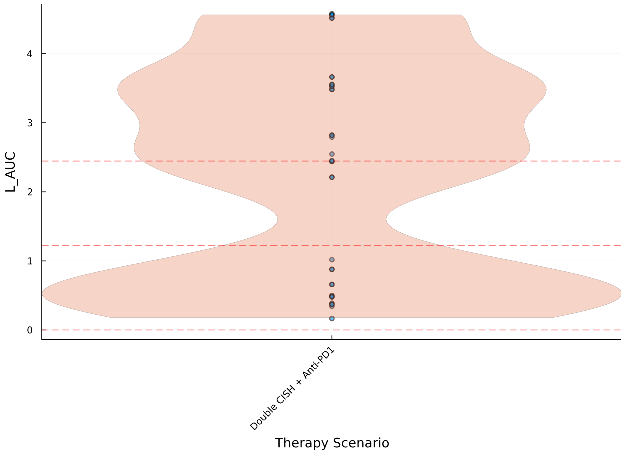
L_AUC Across Therapy Scenarios
