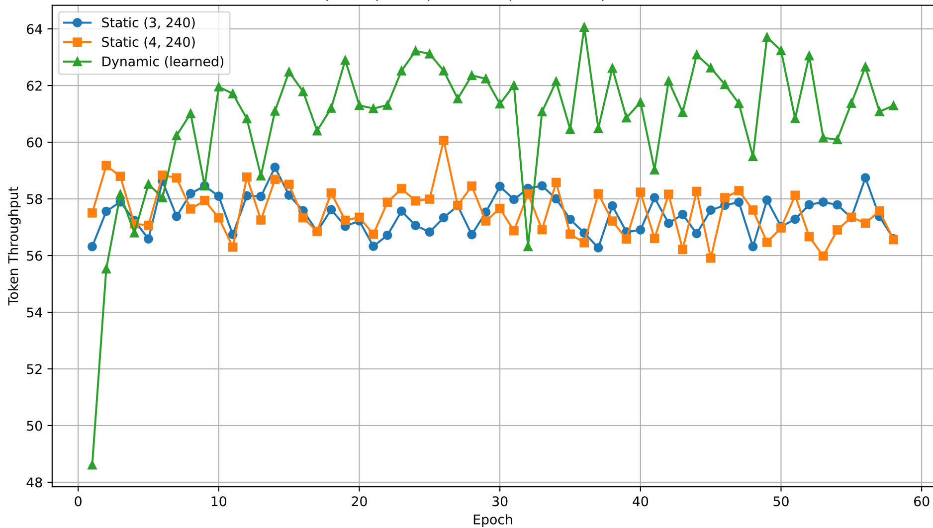
Speedup Comparison (Updated at Epoch 58)
