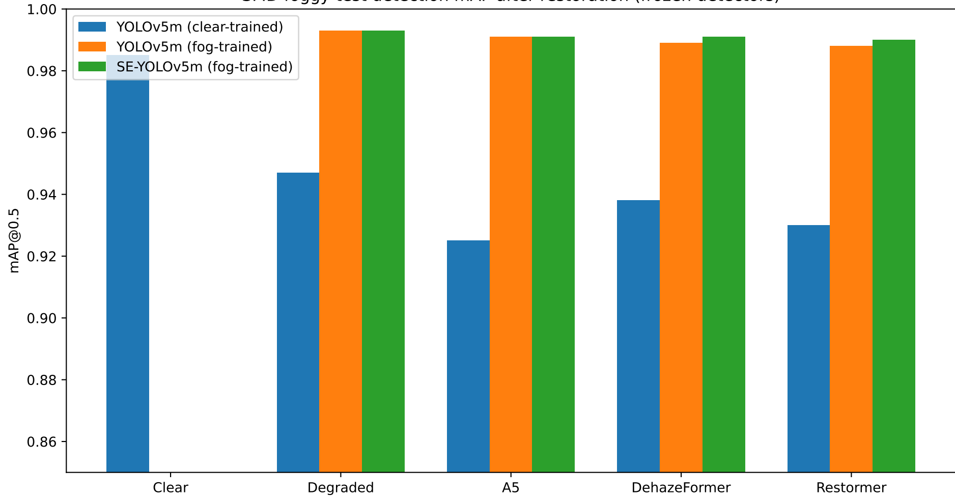
SFID foggy-test detection mAP after restoration (frozen detectors)
