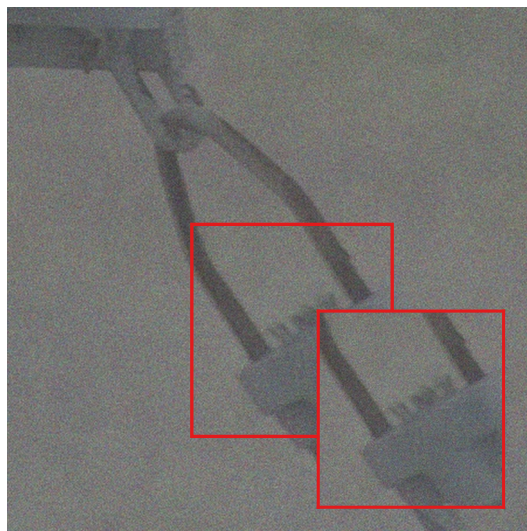
Input 12.20 dB
