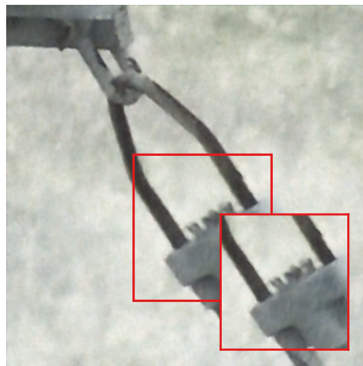
Restormer 22.16 dB
