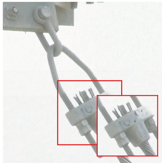
30.46 dB
