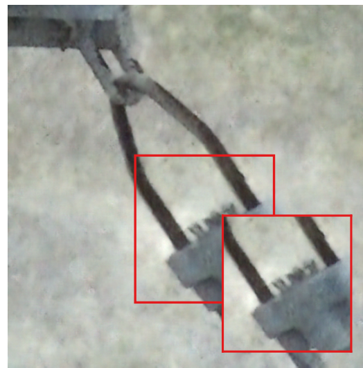
DehazeFormer 27.97 dB
