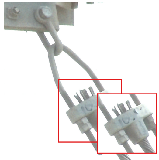
37.28 dB
