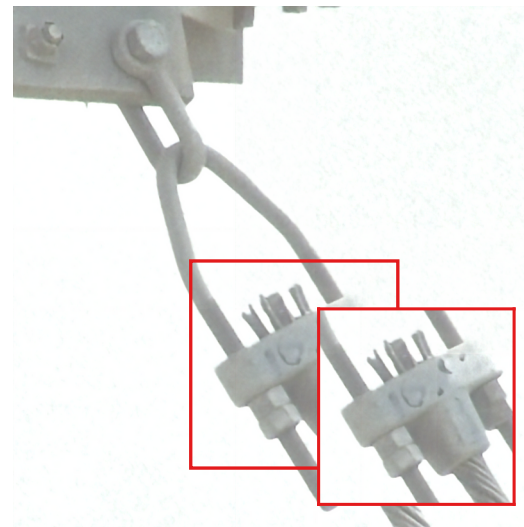
32.63 dB
