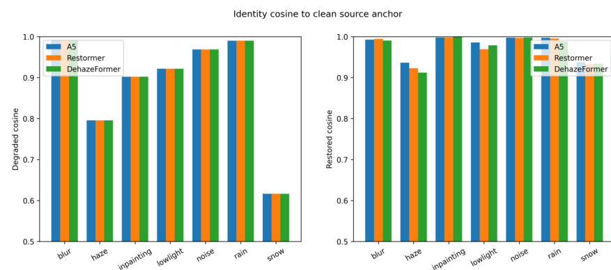
(d) Identity recovery by degradation
