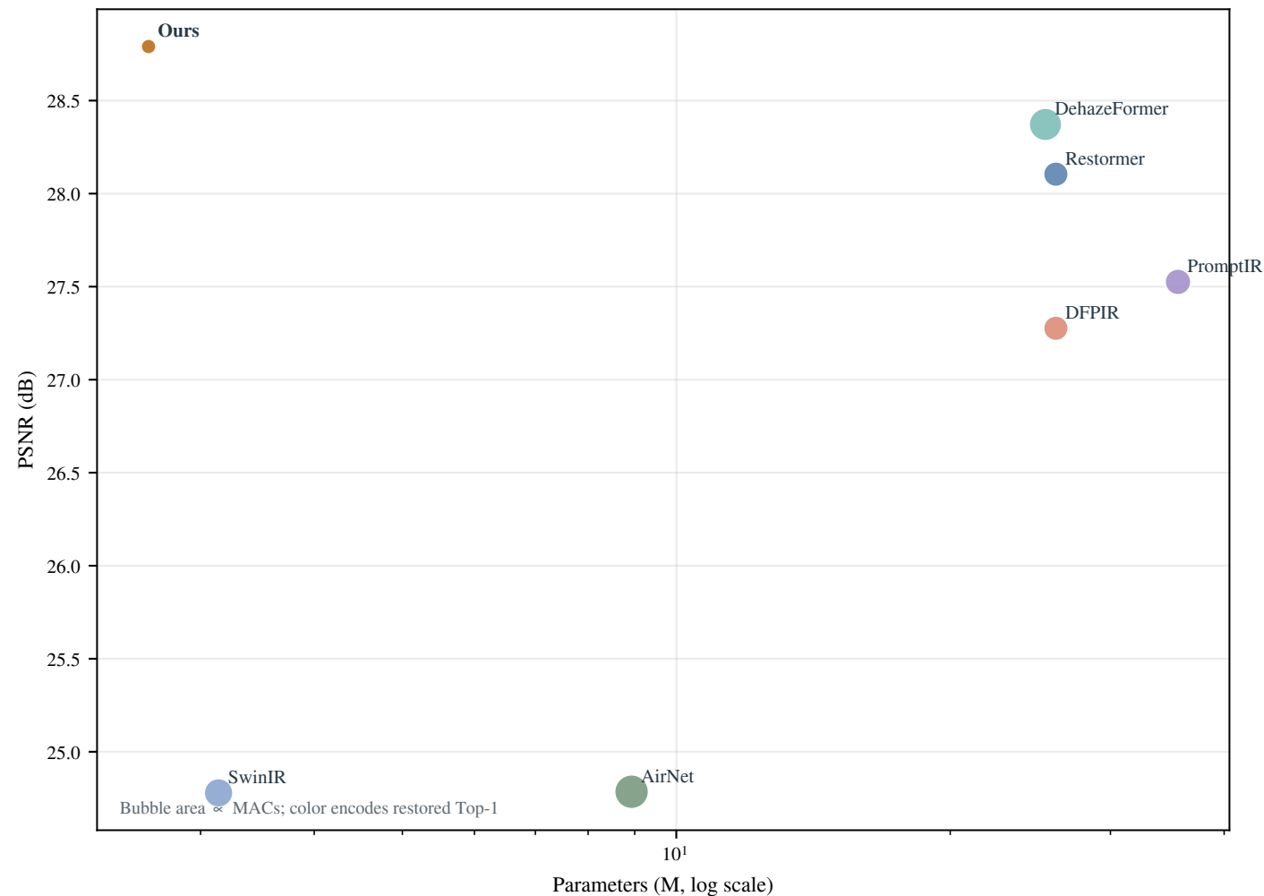
Figure 6. Quality–efficiency–identity Pareto
