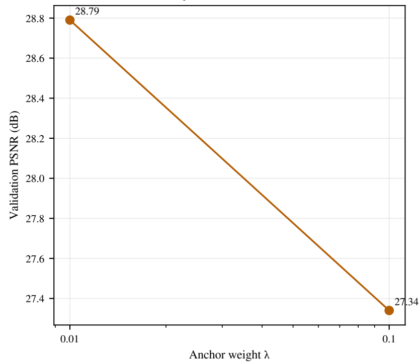
(b) Anchor sensitivity
