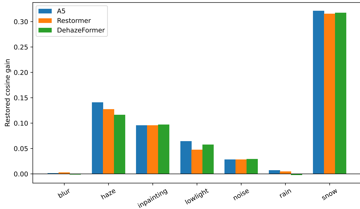
Identity recovery gain across degradations
