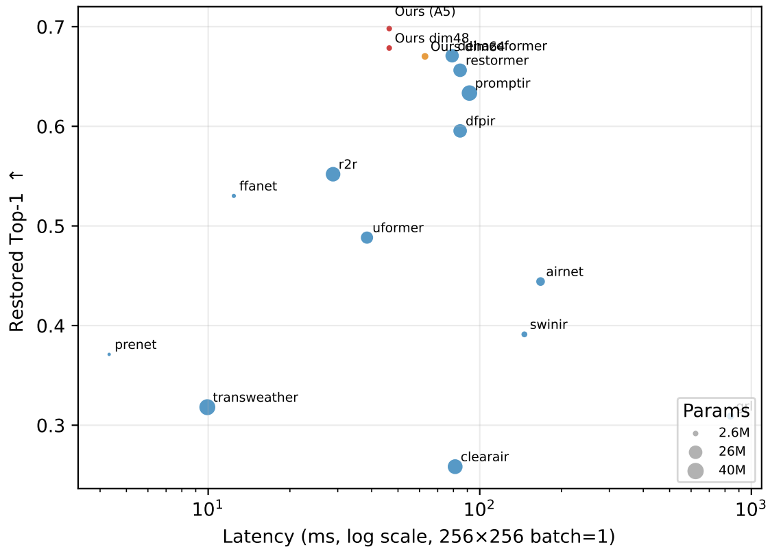
Efficiency vs quality / source retention (latency from project-wide consistent protocol: 256×256, batch 1, fp32, V100)
