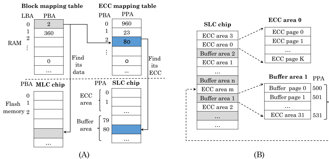
FIGURE 18 Management of block mapping table, ECC mapping table, and buffer area in the technique of Hsiehv et al. 32 A, Both the MLC chip and the ECC mapping table are indexed by PBA. Both the block mapping table and the ECC mapping table are maintained in RAM; B, Buffer areas and ECC areas are physically interchangeable in SLC. However, buffer/ECC pages within the buffer/ECC areas must be physically contiguous
