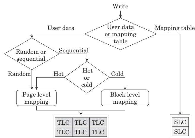
FIGURE 20 Working of the technique of Chang et al 18
