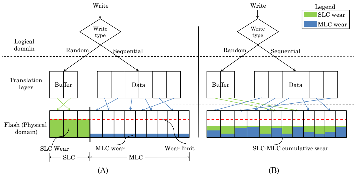
FIGURE 3 (SLC and MLC chips are physically separated. Mapping of random writes to SLC can lead to its early wear out). (Only MLC blocks are used, some of which can be selectively programmed as SLC to improve performance and achieve wear leveling). 25 A, Hard partitioning; B, Soft partitioning
