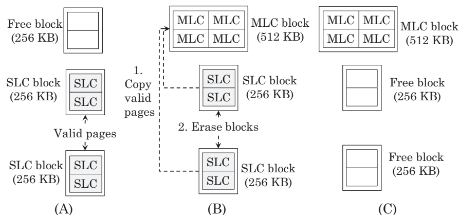
FIGURE 8 Free-space reclamation in the technique of Lee et al. 48 A, Initial state; B, Copy & erase; C, Final state
