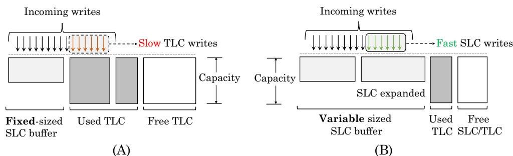
FIGURE 6 Fixed-sized SLC buffer versus variable-sized SLC buffer approach 39 A, Fixed-sized SLC buffer techniques; B, Variable-sized SLC buffer techniques
