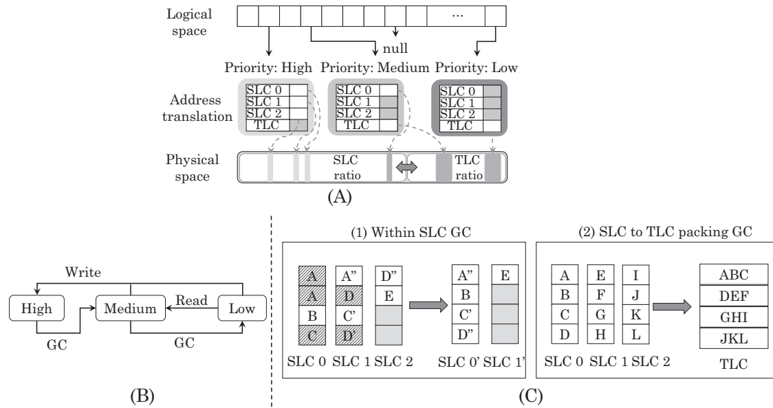
FIGURE 7 Illustration of A, block mapping, B, priority transition, and C, GC operations in the technique of Yang et al. 39 A, Utilization-aware block mapping scheme; B, Priority transition of logical blocks; C, Two types of GC operations for low and high utilization cases, respectively
