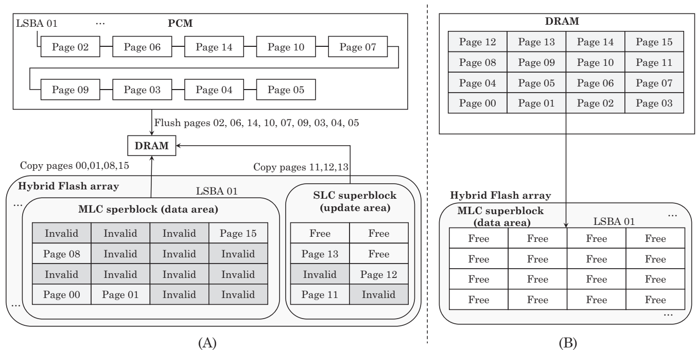
FIGURE 13 Illustration of flush operation in technique of Lu et al. 42 A, Valid pages are gathered from PCM, data area, and update area for flushing to DRAM; B, The pages stored in DRAM are sorted and transferred into data area and the original updated data area is erased
