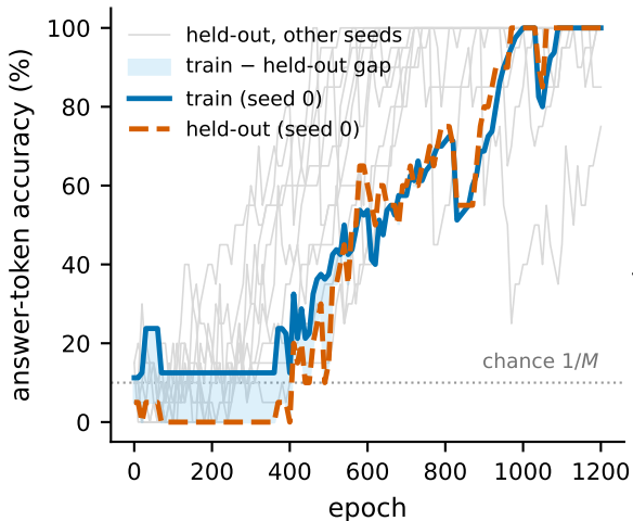
Chance plateau, then a seed-timed transition
