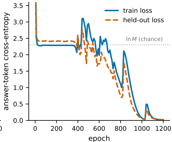
Loss plateau at \ln M , then collapse
