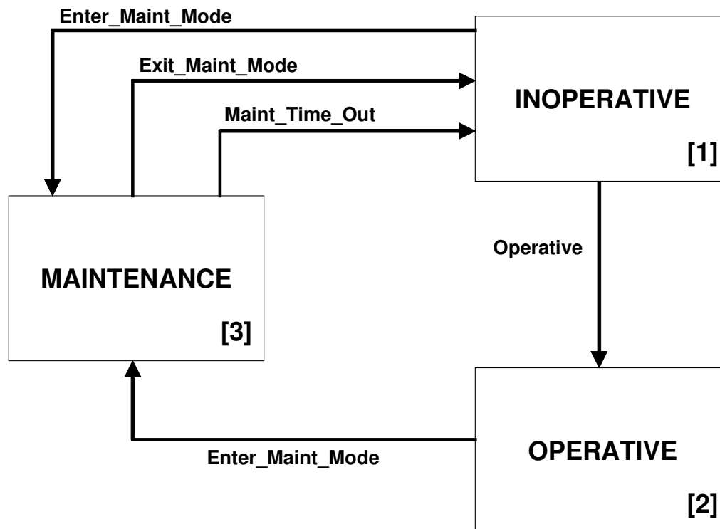
Figure 3 : Tank Probe State Diagram
