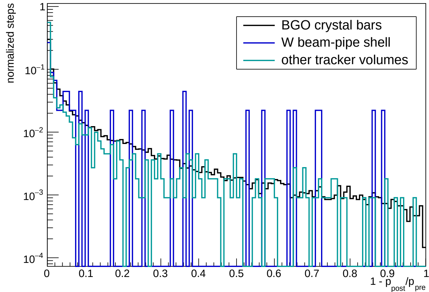
Primary eBrem fractional energy loss, shape-normalized
