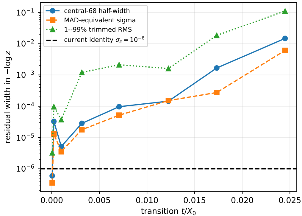
No-eBrem transition location and straggling
