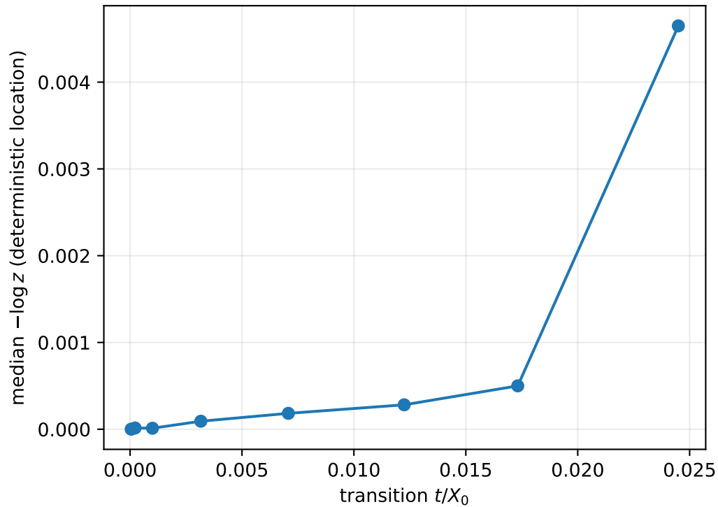
No-eBrem transition location and straggling
