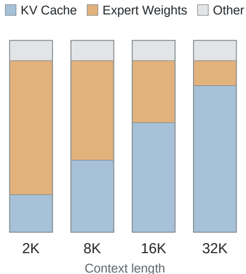
(b) HBM Capacity Competition
