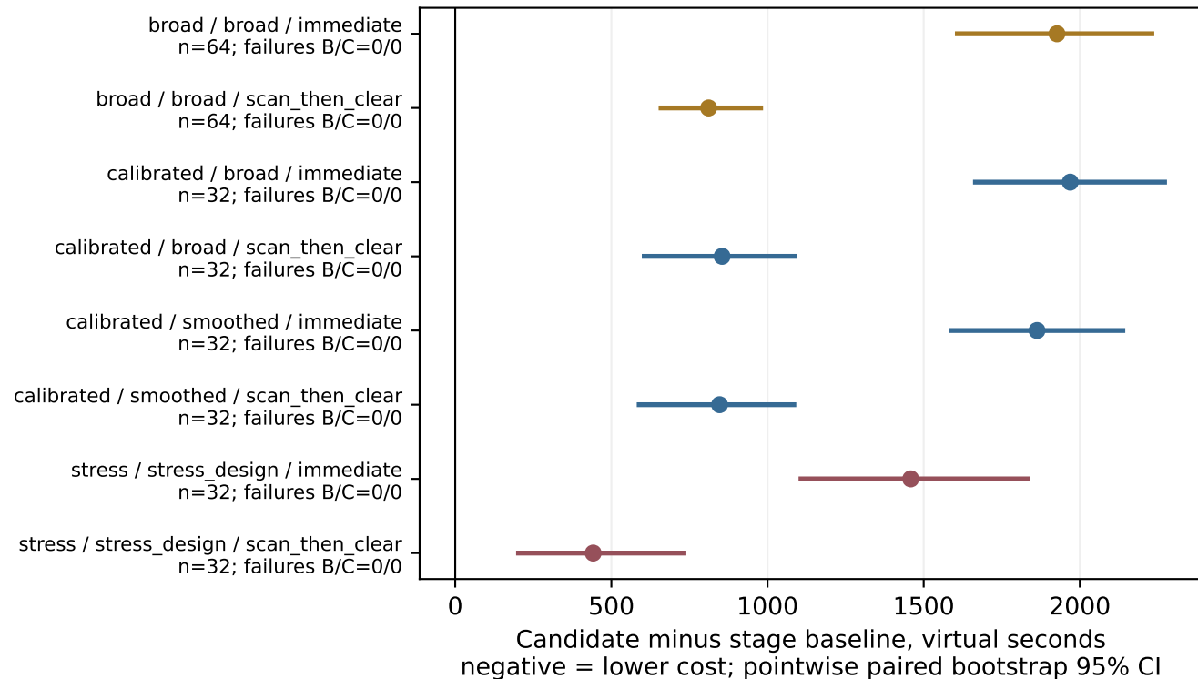
P4: development
