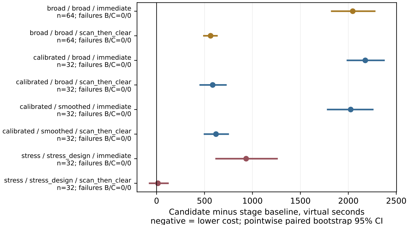
P3: development
