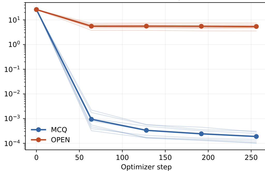
D Common MCQ CE probe
