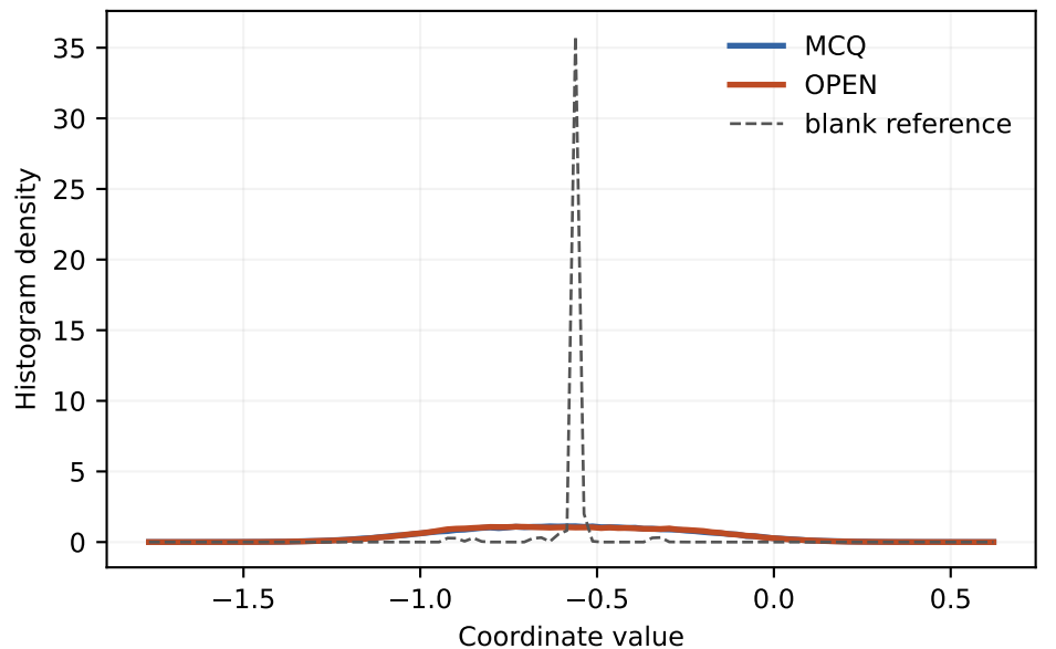
Latent channel 3
