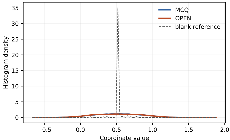
Latent channel 3
