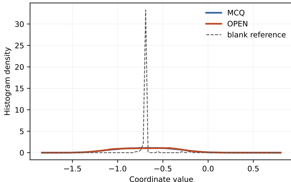
Latent channel 2
