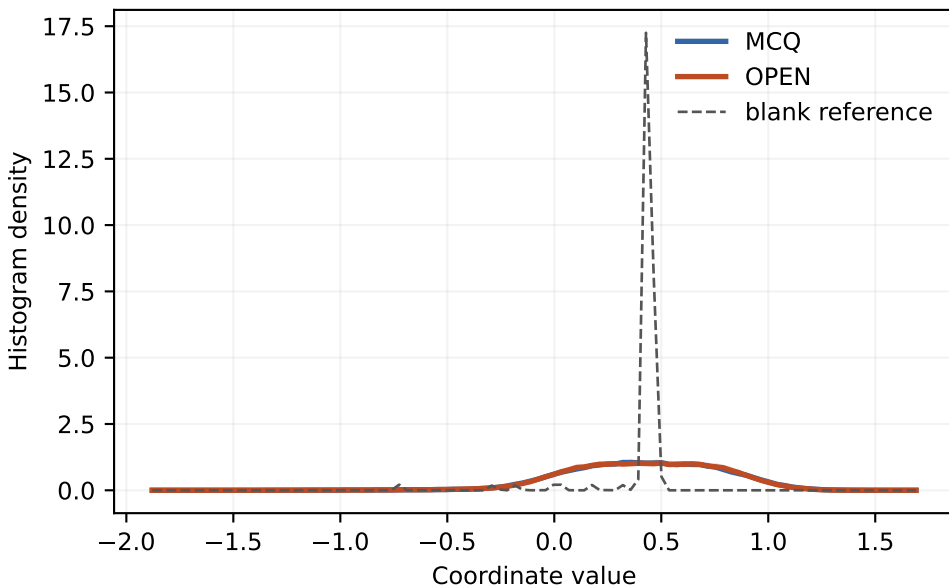
Latent channel 2
