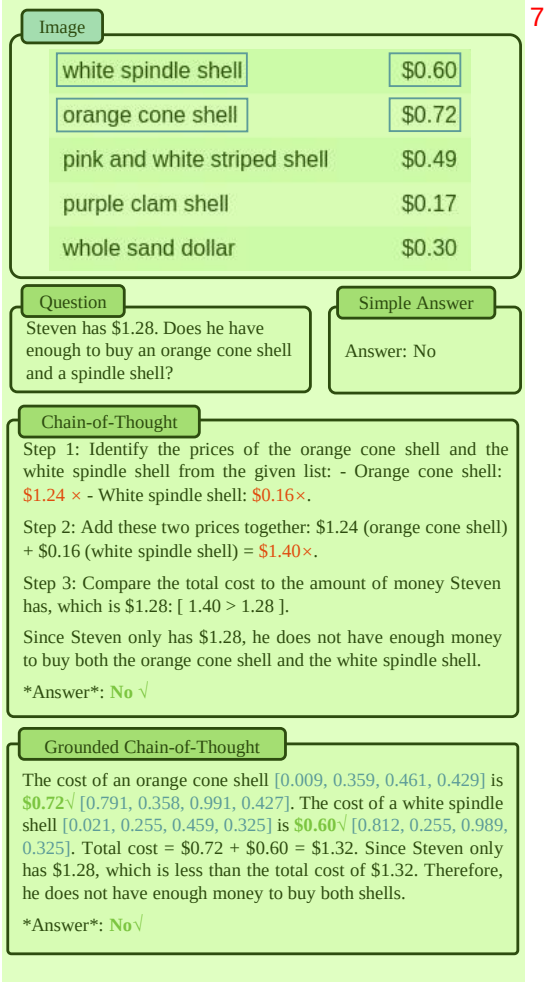
Figure 1. Comparison between normal and grounded Chain-of-Thought (CoT). The normal CoT contains factual errors, despite giving the correct answer. In addition to reasoning, the grounded CoT (GCoT) uses bounding boxes to ground key information in the image, which can be self-verified by the model and help minimize factual errors.
