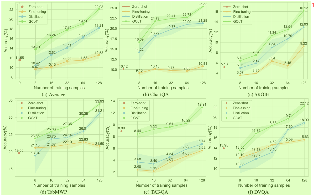
Figure 3. Main results on the five specialized vision datasets. Fine-tuning means directly fine-tuning the model with simple question-answer pairs. Distillation means training the model with LLaMA distilled CoT data. All training-based methods are based on the same backbone and the LoRA method. Overall, the performance of GCoT surpasses the fine-tuning and distillation methods across all datasets and sample sizes. The shadow areas represent variance.
