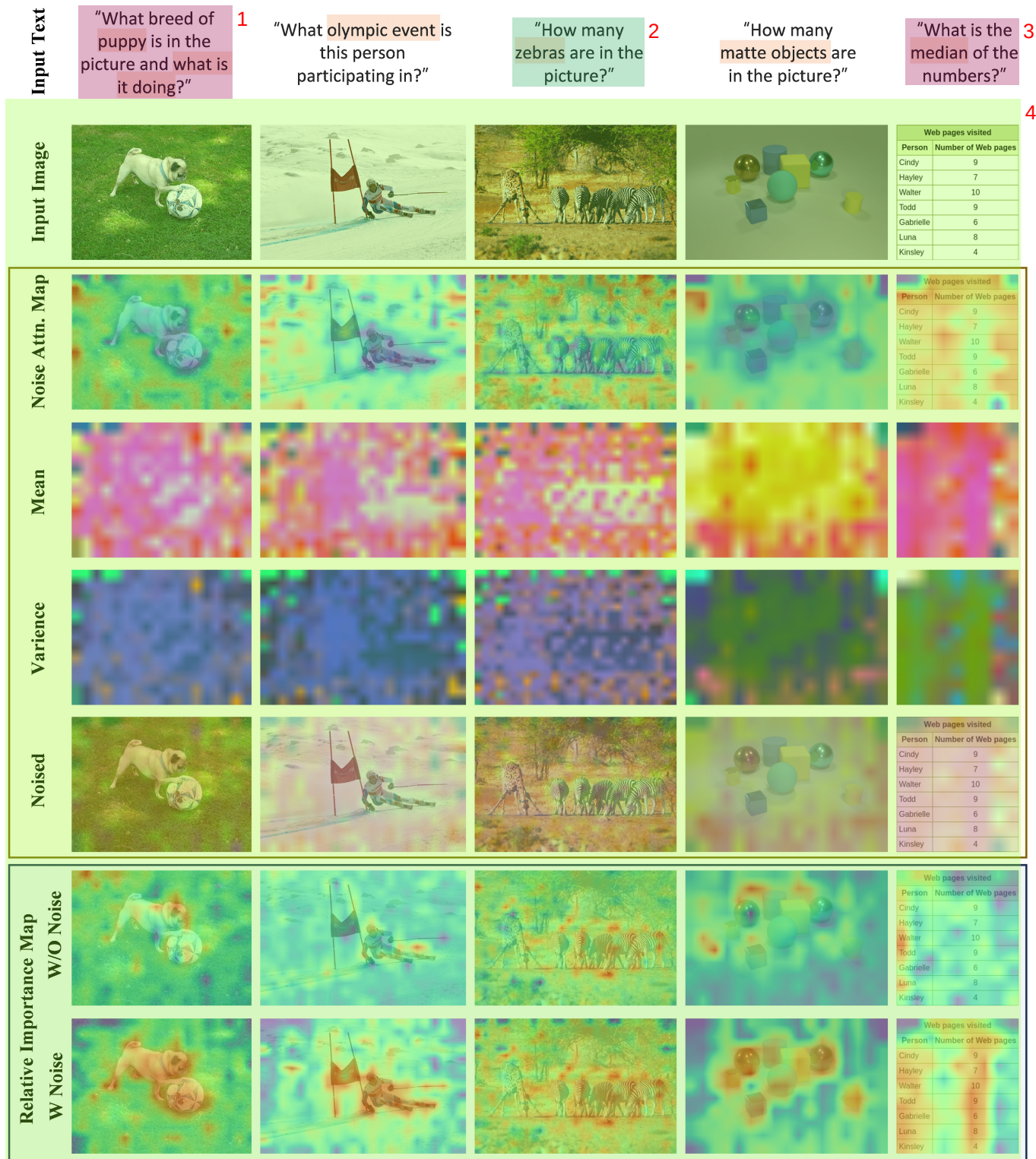
Figure 3: Visualization of generated noise injected into high-dimensional visual features. 5
