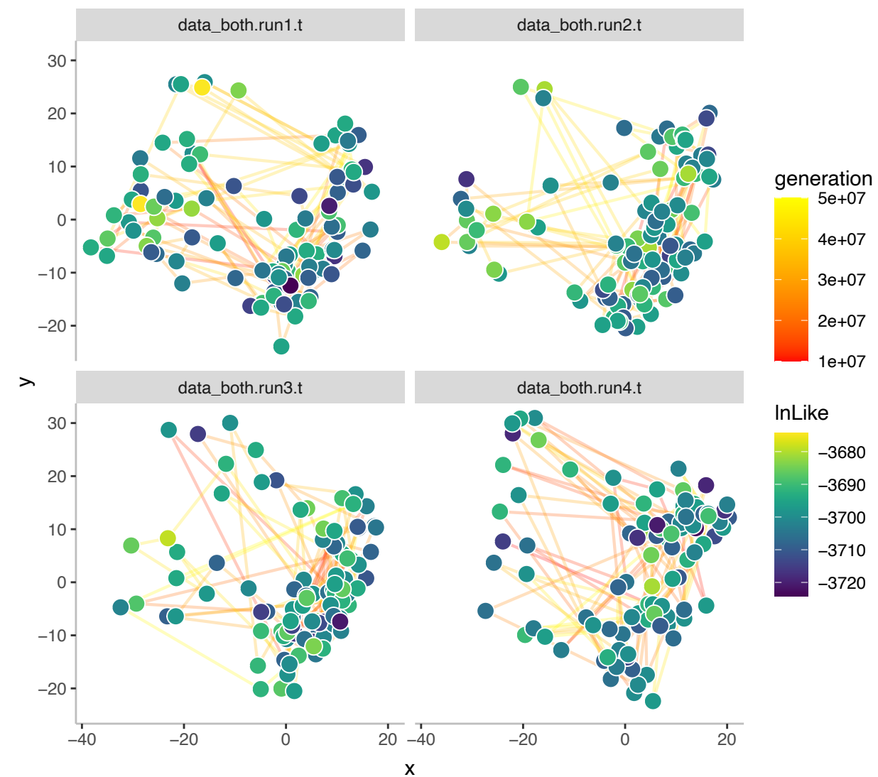
C. Continuous+Discrete, Unlinked WN Clock
