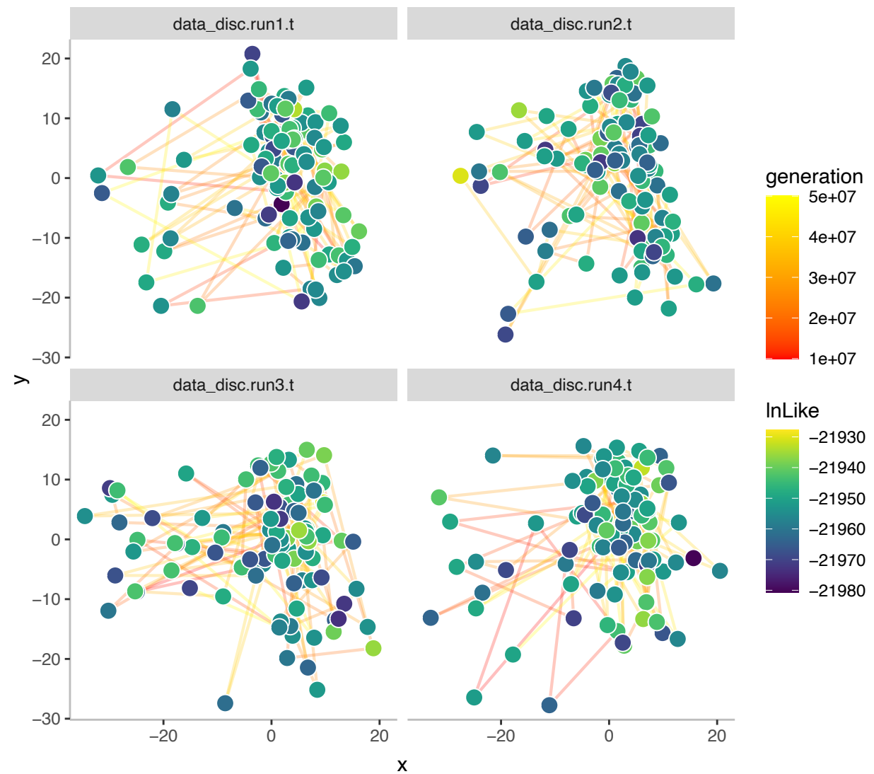
D. Discretized+Discrete, Unlinked WN Clock
