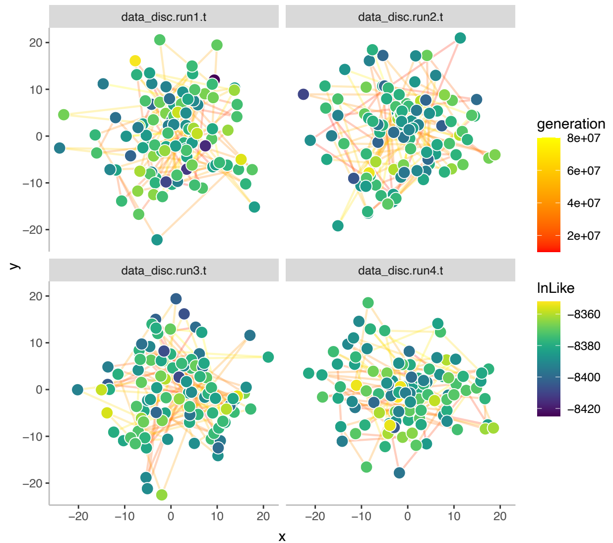
D. Discretized+Discrete, Unlinked ILN Clock
