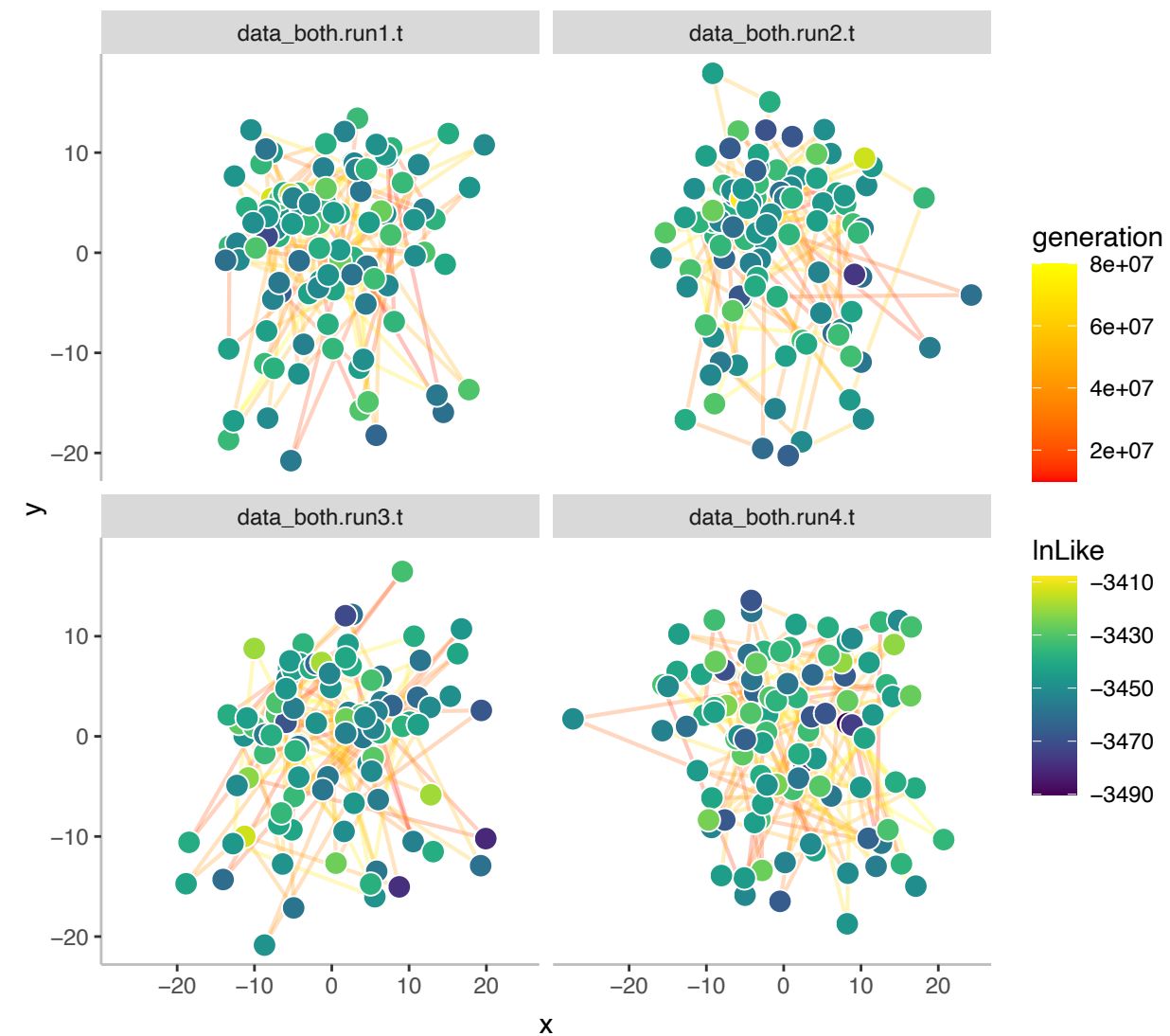
C. Continuous+Discrete, Unlinked ILN Clock
