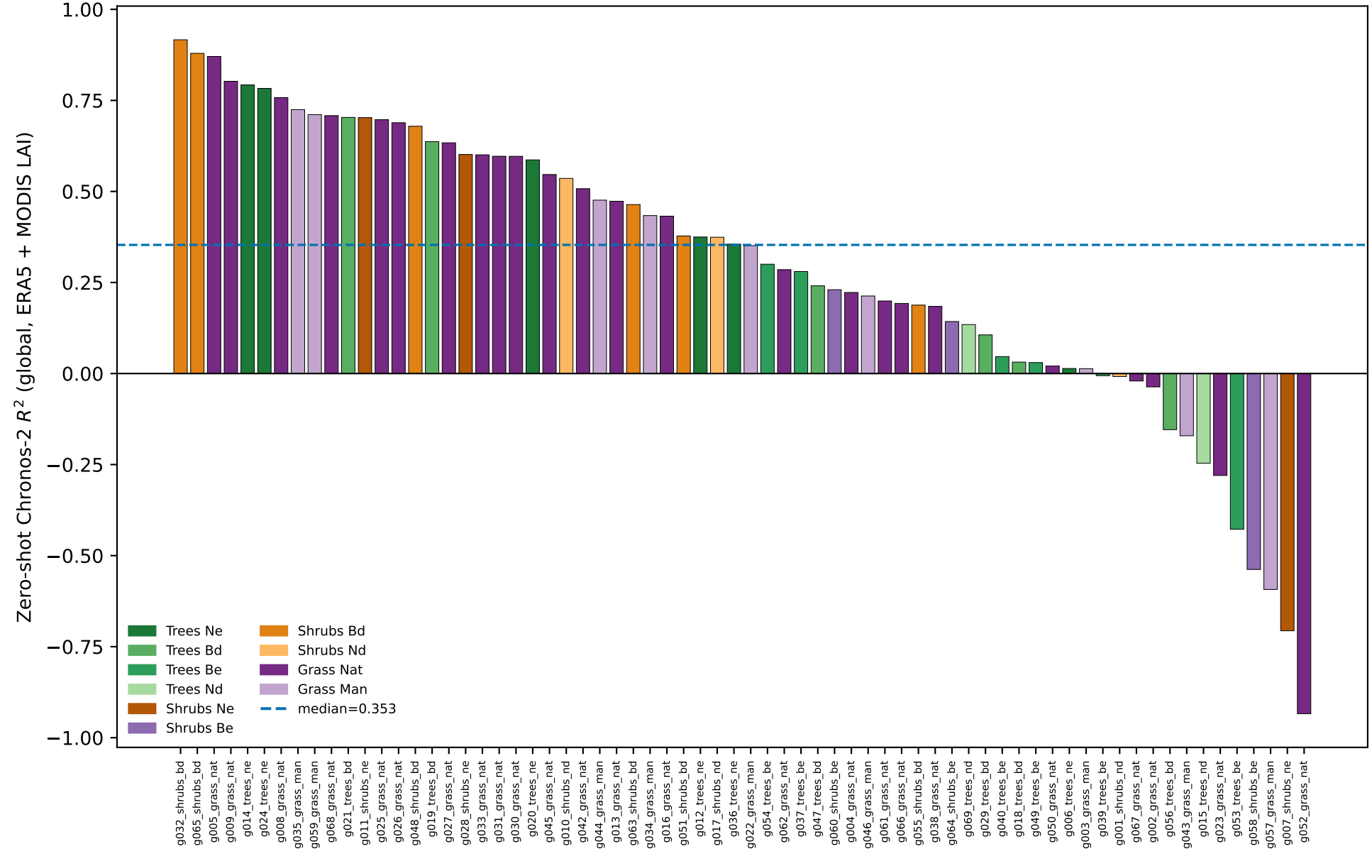
(a) All 68 usable pixels, sorted by R^2
