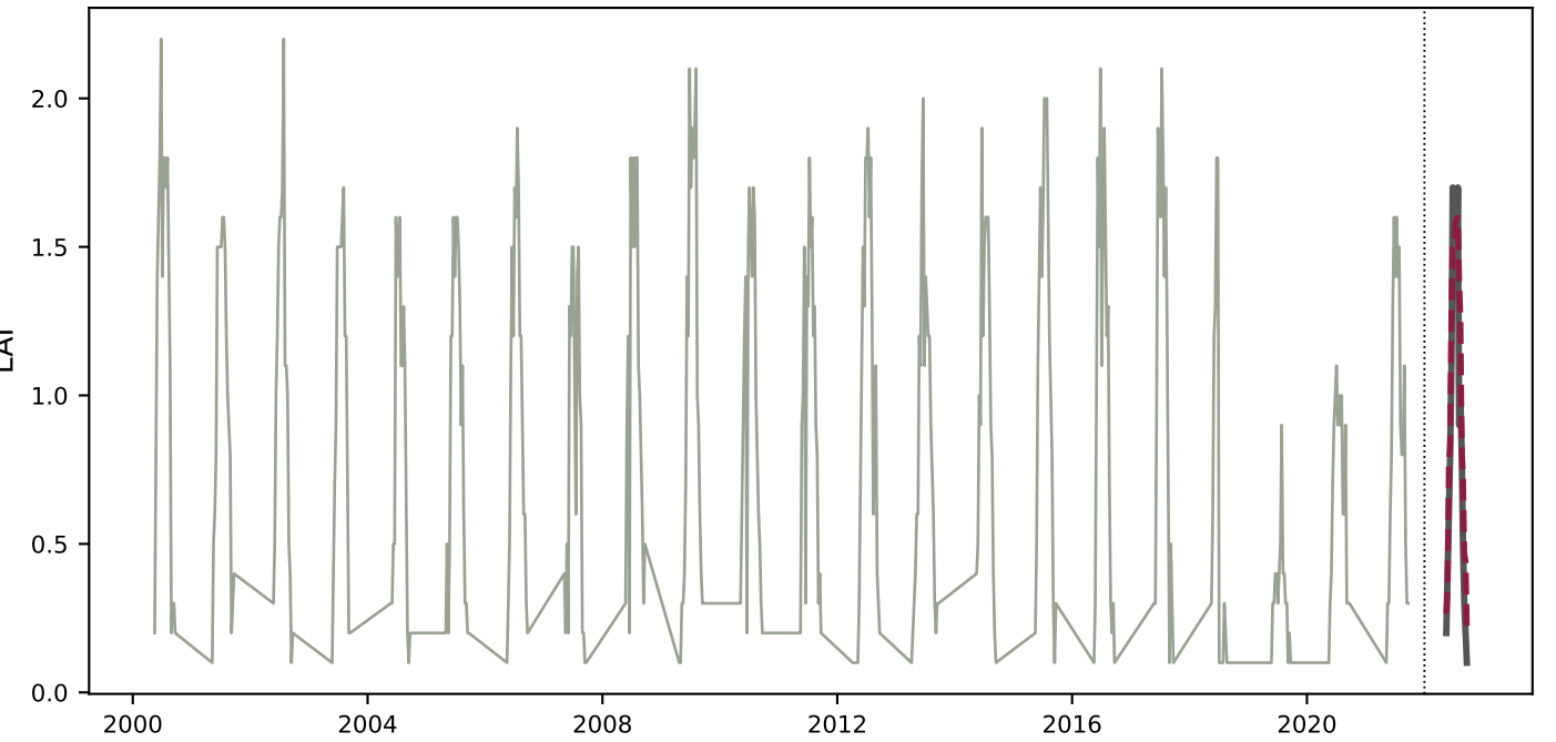
g014_trees_ne — Siberia / Boreal Eurasia evergreen forest R^2=0.793 , Pearson r=0.897 , context=472 steps
