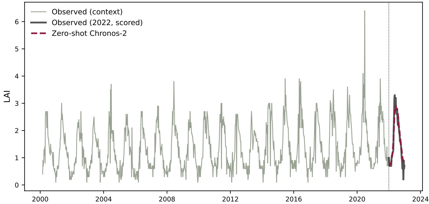
g005_grass_nat — Siberia / Boreal Eurasia grassland R^2=0.871 , Pearson r=0.956 , context=369 steps
