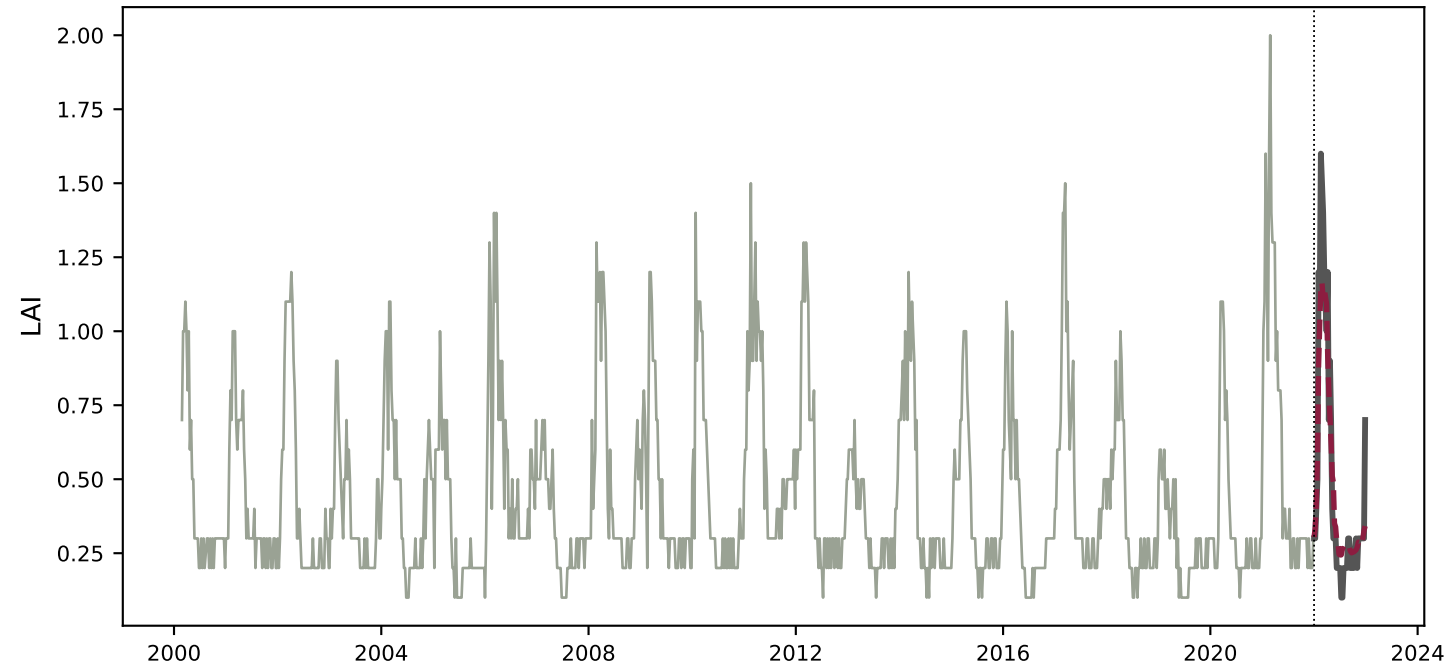
g009_grass_nat — Canada grassland R^2=0.802 , Pearson r=0.910 , context=451 steps
