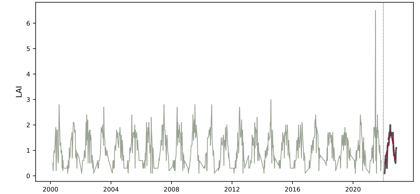
g068_grass_nat — Southern S. America grassland R^2=0.708 , Pearson r=0.855 , context=971 steps
