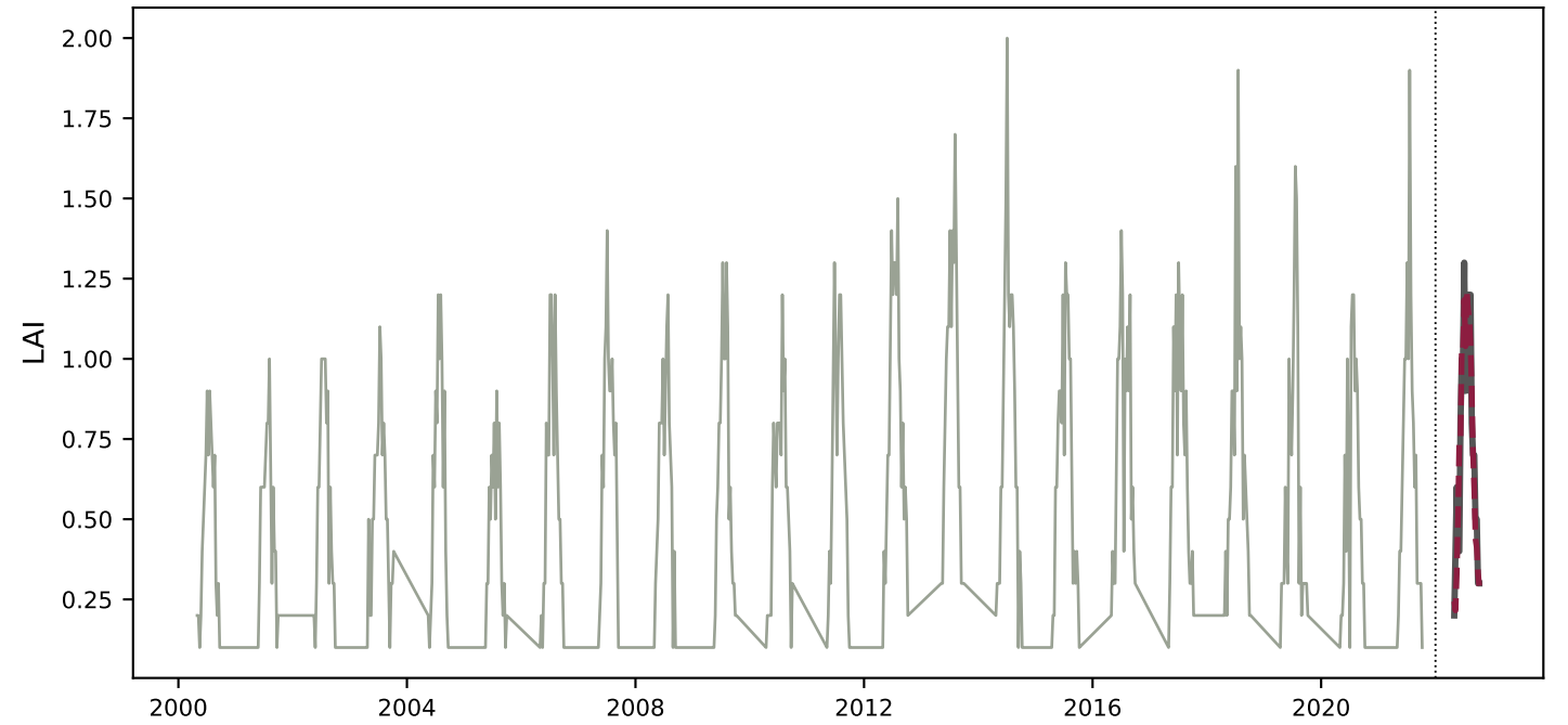
g024_trees_ne — Western Europe evergreen forest R^2=0.783 , Pearson r=0.886 , context=747 steps
