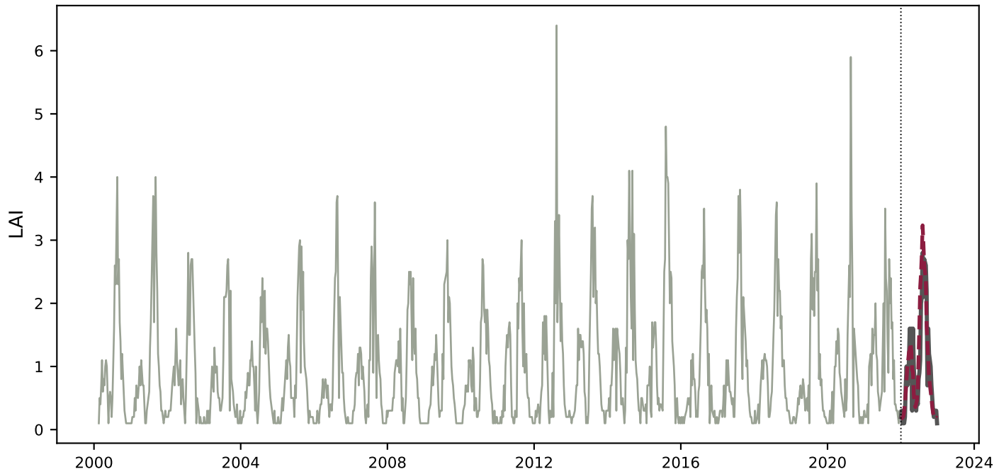
g035_grass_man — East Asia managed grassland R^2=0.724 , Pearson r=0.885 , context=967 steps
