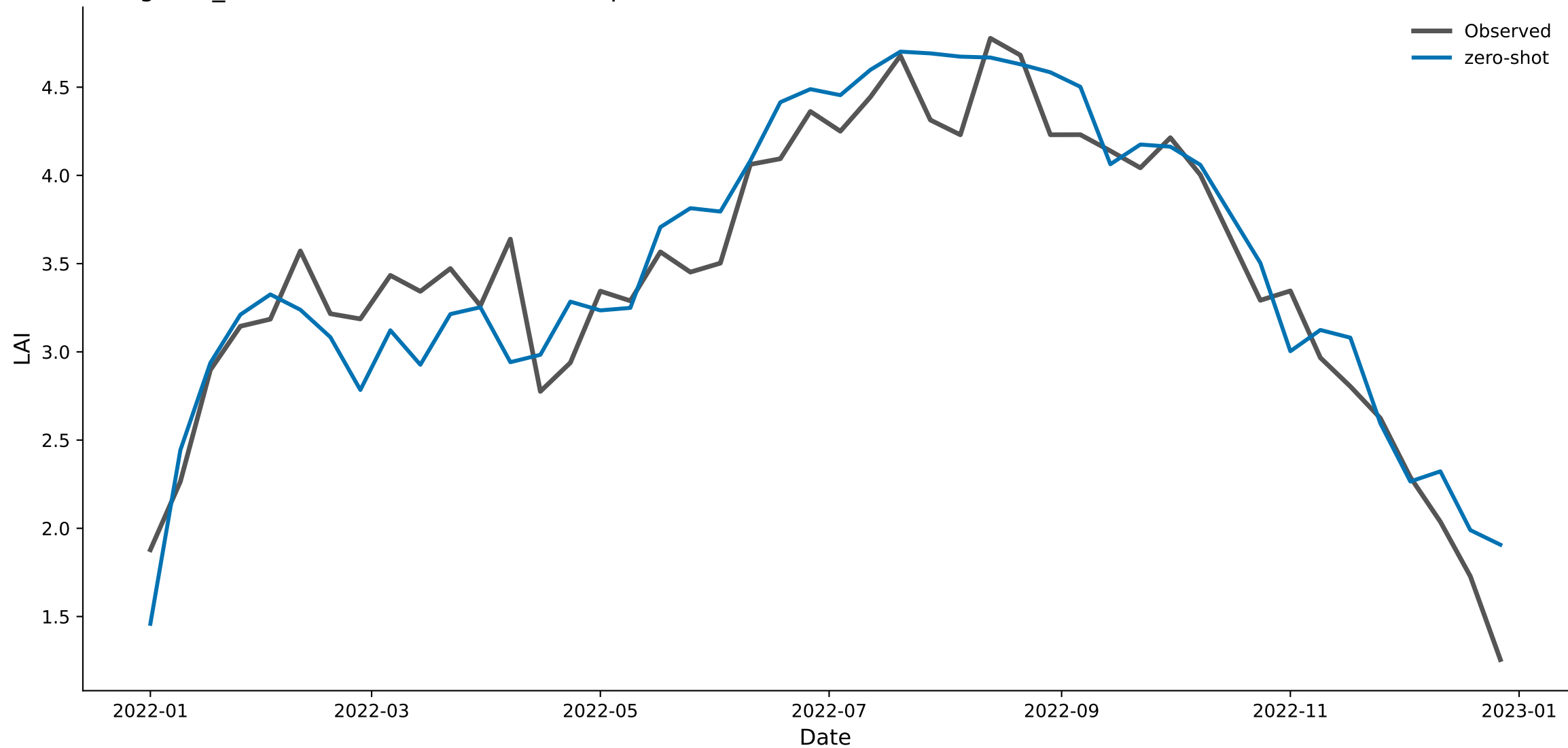
evergreen_west — Chronos-2 (zero-shot) predicted vs. observed LAI, 2022
