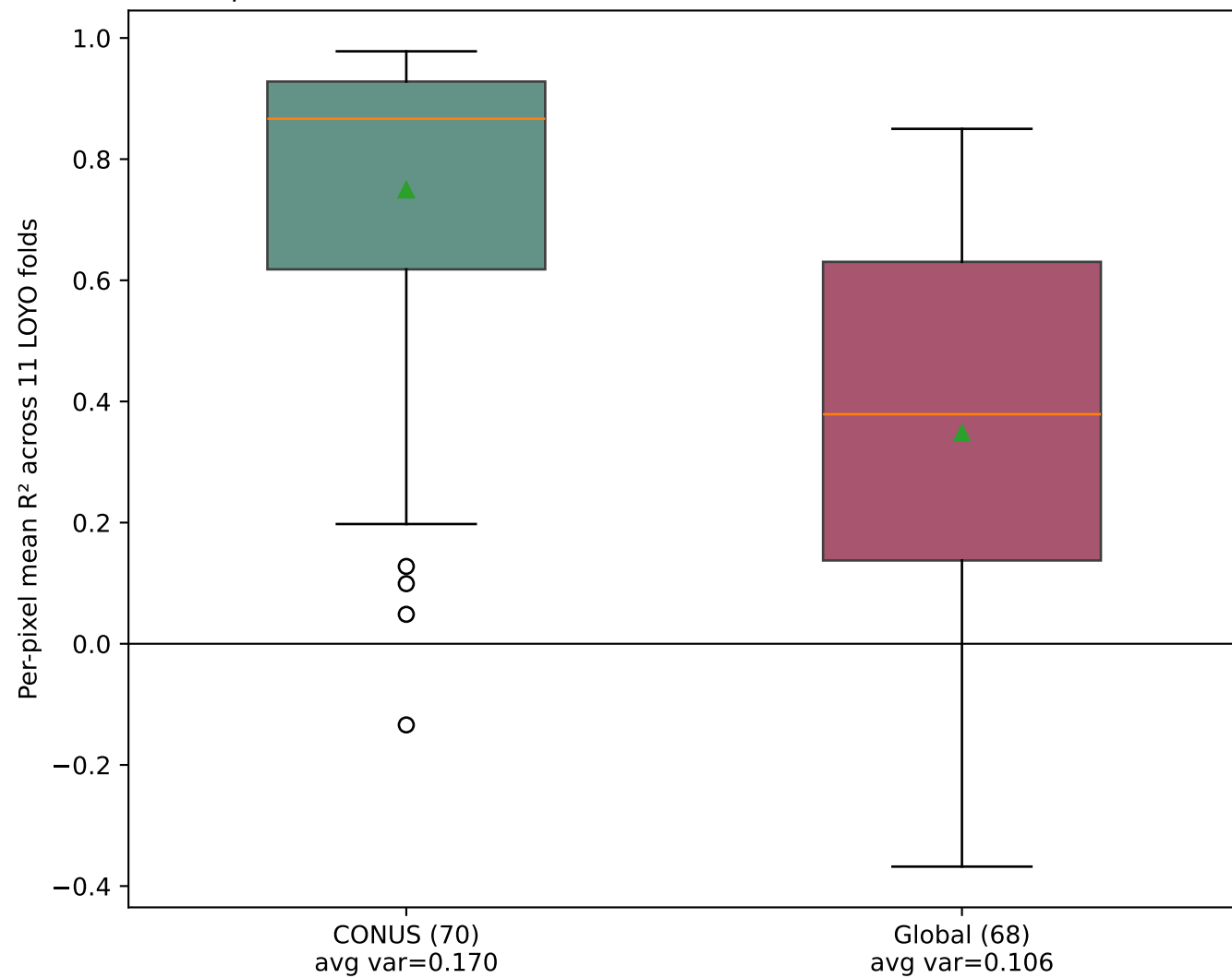
(a) Per-pixel mean R^2 (LOYO-CV, 2012-2022)
