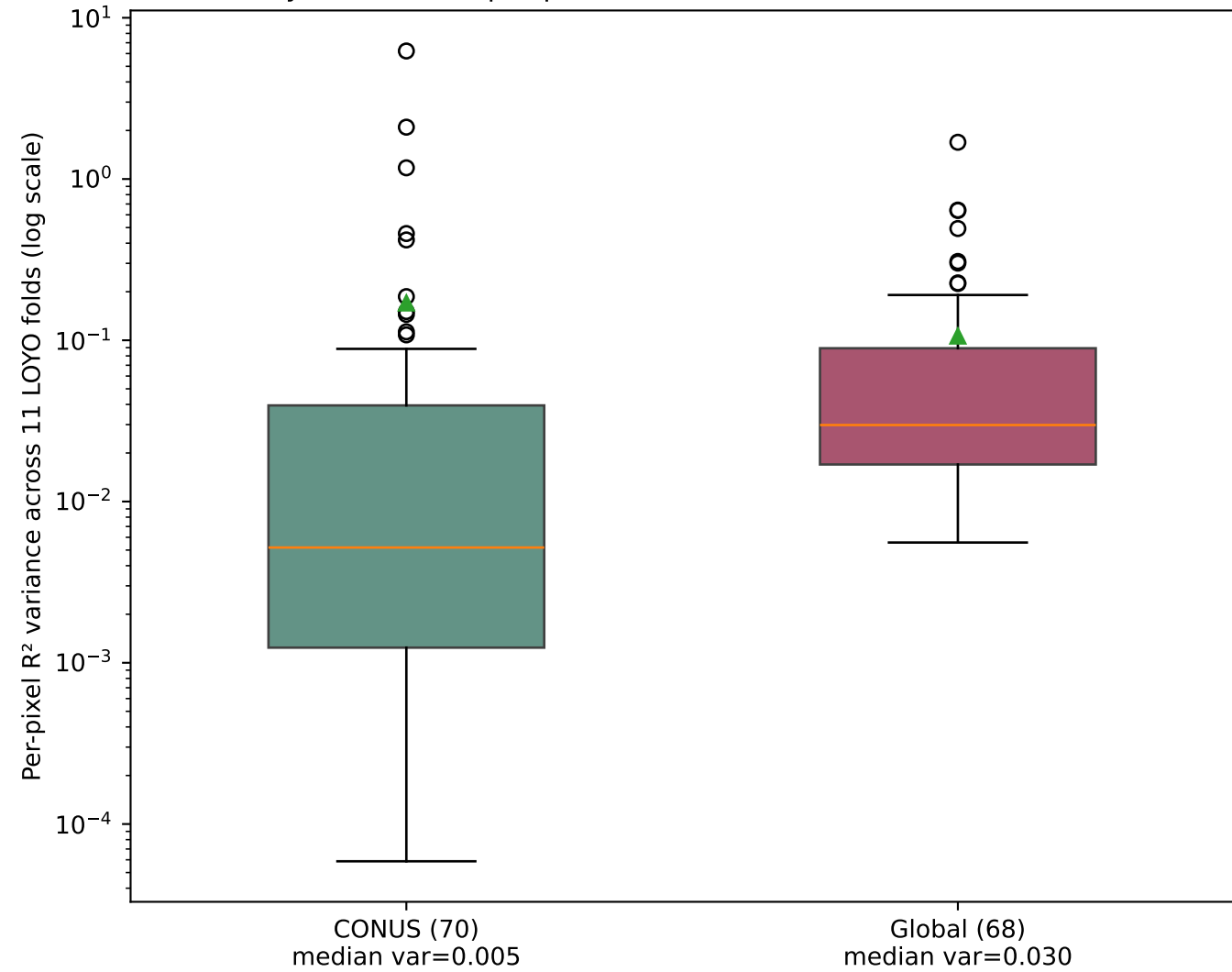
(b) Year-to-year variance per pixel (lower = more stable)
