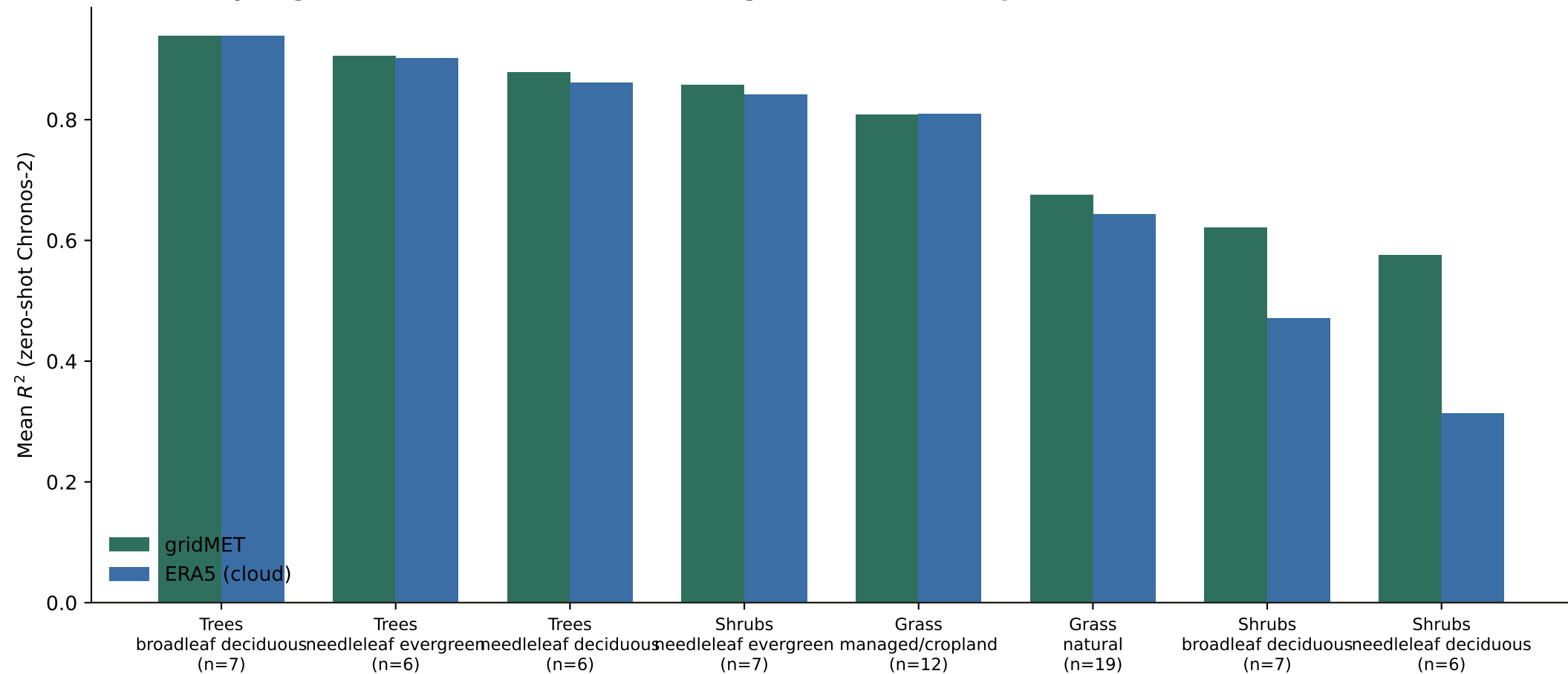
Mean R^2 by vegetation class: ERA5 (cloud) vs. gridMET, same 70 pixels
