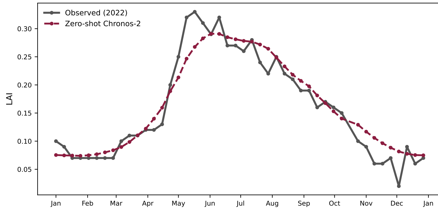
g009_grass_nat — Solid: Canada grassland R^2=0.802 , Pearson r=0.910
