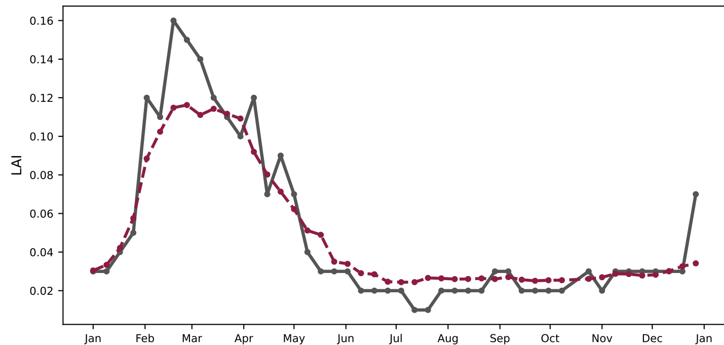
g009_grass_nat — Canada grassland R 2 =0.802, Pearson r=0.910
