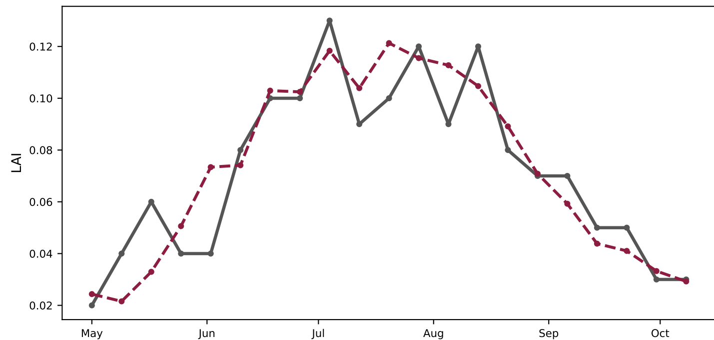
g024_trees_ne — Western Europe evergreen forest R 2 =0.783, Pearson r=0.886
