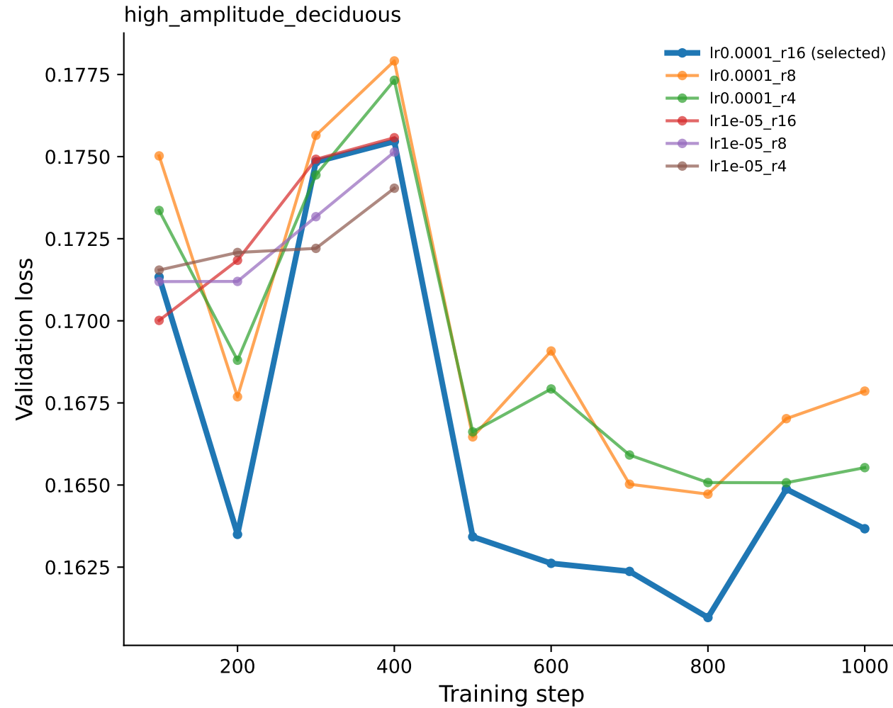
All 6 searched configurations' validation loss, per pixel
