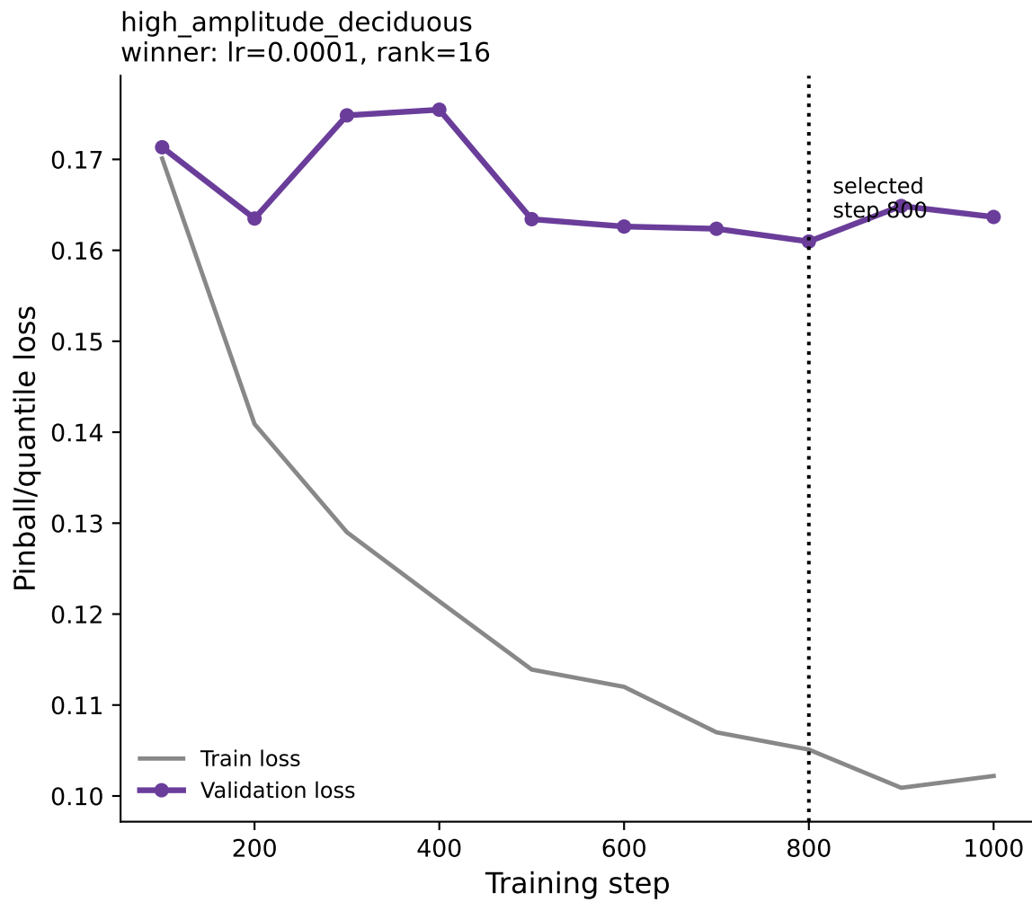
Winning configuration per pixel: train vs. validation loss (dotted line = selected checkpoint)
