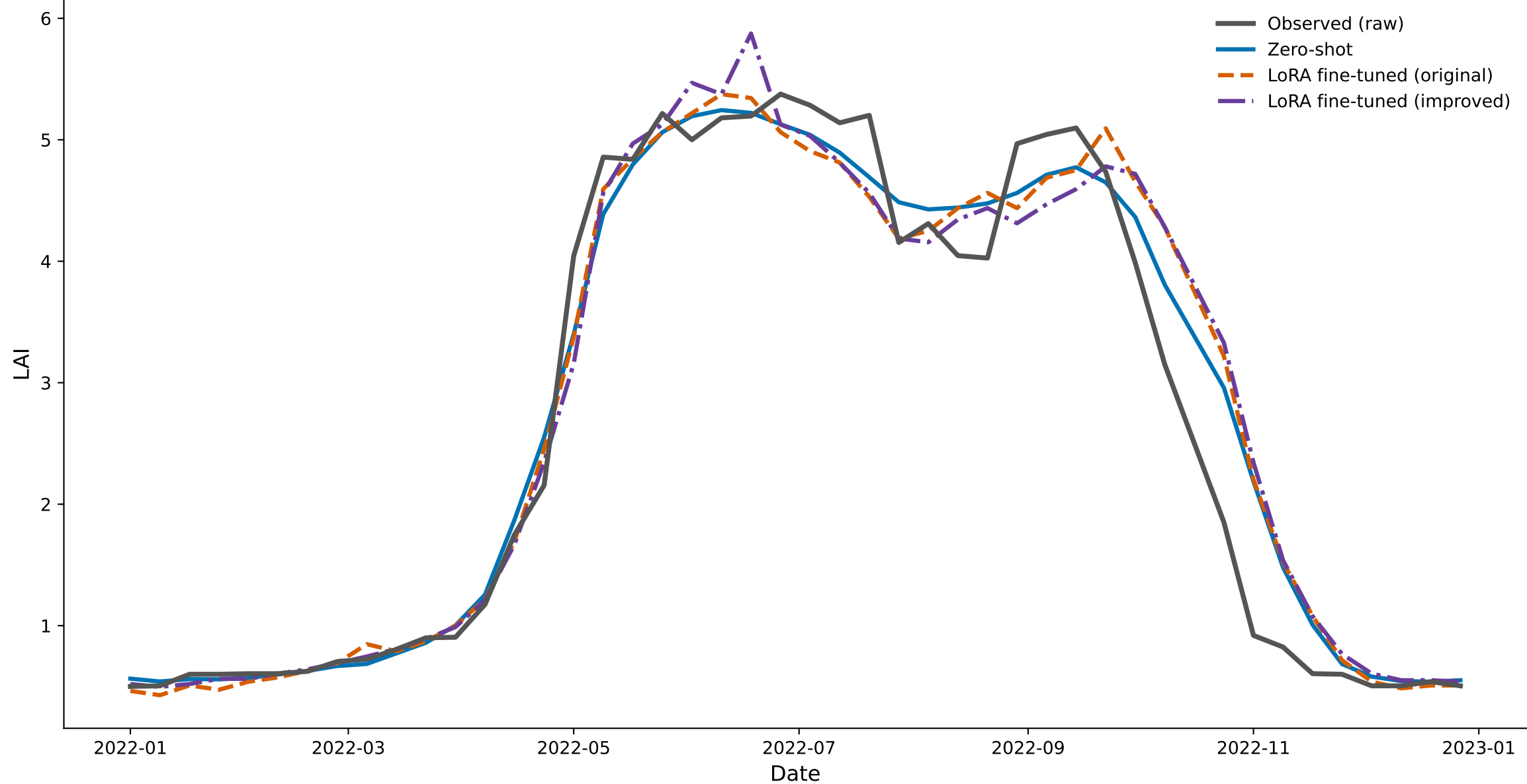
high_amplitude_deciduous — zero-shot vs. original vs. improved LoRA fine-tuning, 2022
